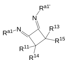
Structure 3f
