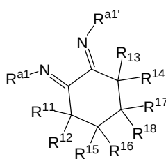
Structure 5f
