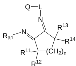
Structure 15f
