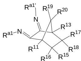
Structure 6f
