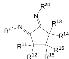
Structure 4f
