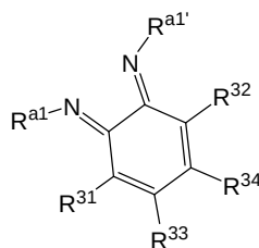
Structure 7f
