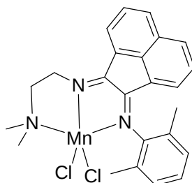
Structure XXII
