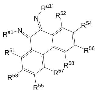
Structure 12f
