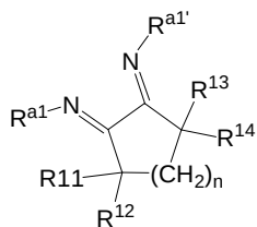
Structure 2f
