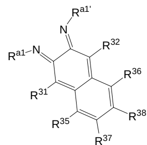
Structure 8f
