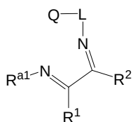
Structure 14f
