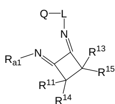
Structure 16f
