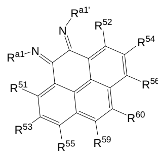
Structure 13f
