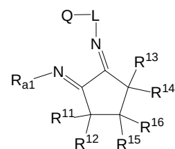
Structure 17f
