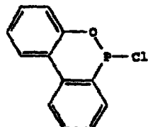
6-Chloro-6H-dibenz[c,e][1,2]oxaphosphorin
