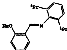
25 salicylaldehyde-2,6-diisopropylanilineimine sodium salt
