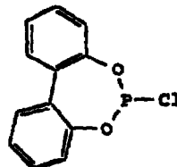
1,1'-biphenyl-2,2'-diylphosphorochloridite
