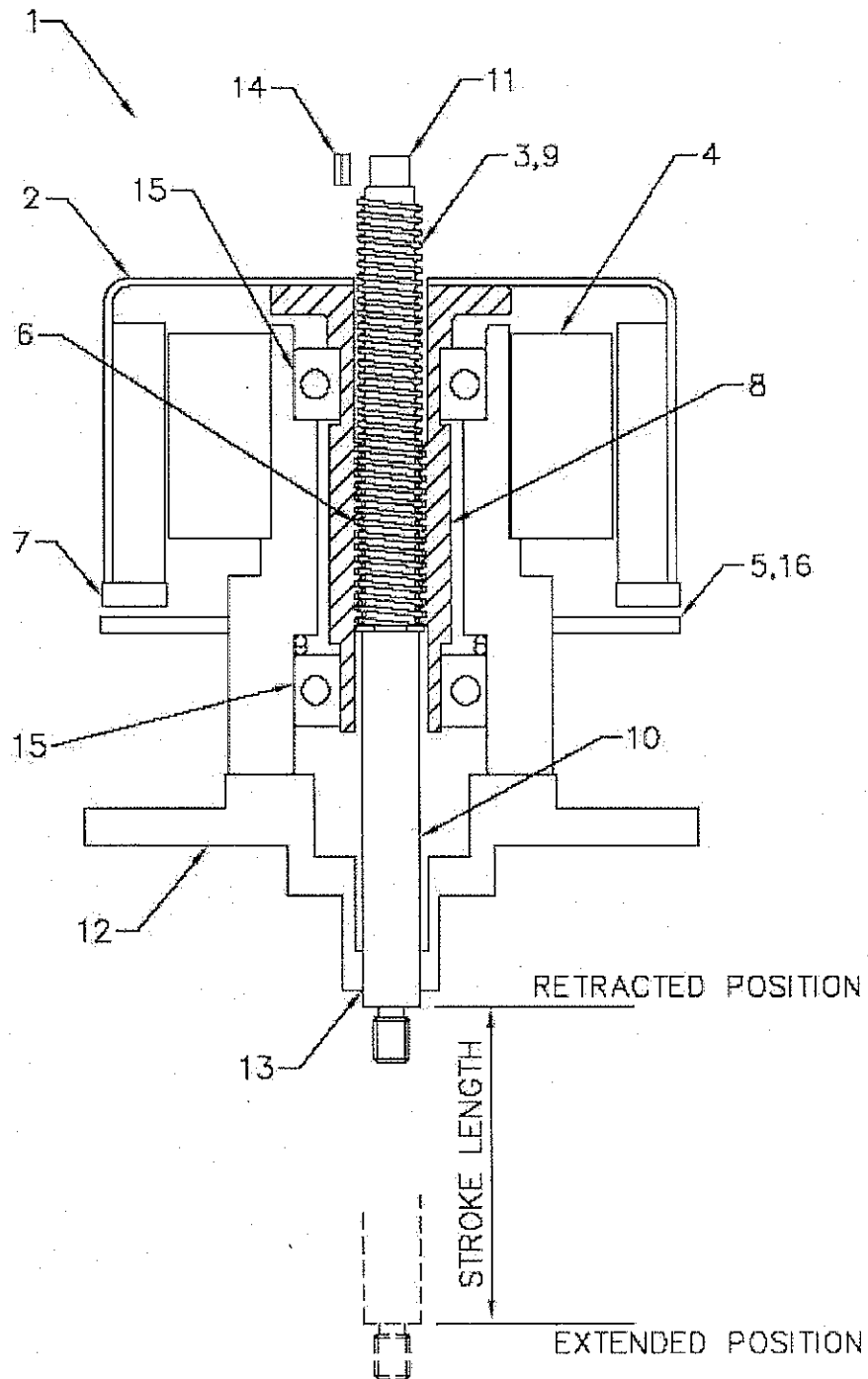
Drawing 1. Cross-sectional view of the linear actuator.
