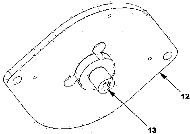
Drawing 5. Anti-rotation hole feature of the mounting plate
