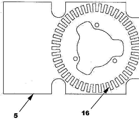
Drawing 6. Tach pattern on the printed circuit board
