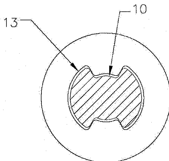
Drawing 3. Close-up view of the anti-rotating shaft with anti-rotational cross section (shaded) 10 inside the hole of the mounting plate that has a matching anti-rotational profile 13 .
