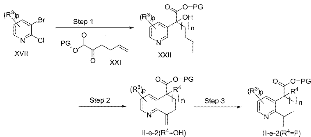
Scheme 17
