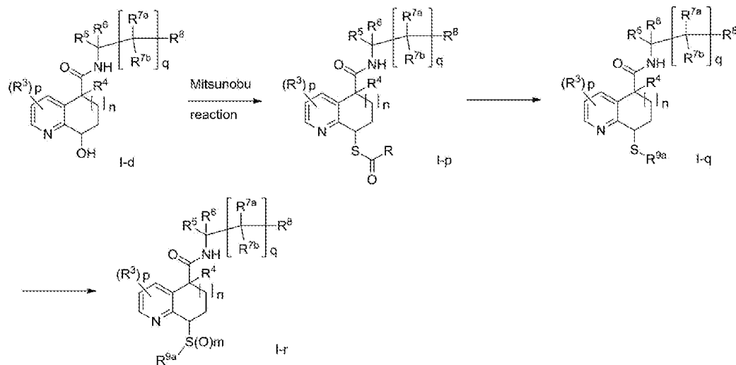
Scheme 13
