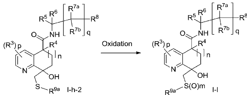
Scheme 10
