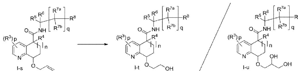
Scheme 14
