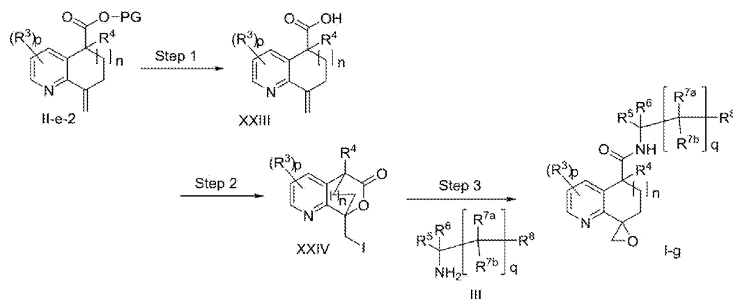
Scheme 18
