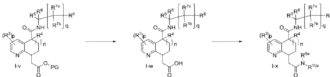
Scheme 15
