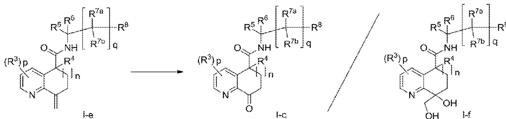
Scheme 7
