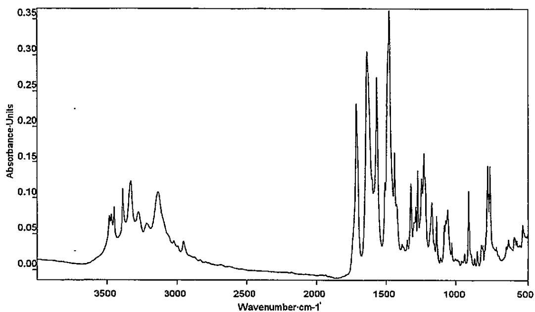
Fig. 3: IR spectra of modifications I-IV, the mesomorphous form and the amorphous form
