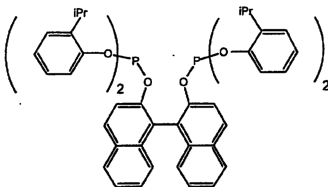
Ligand C
