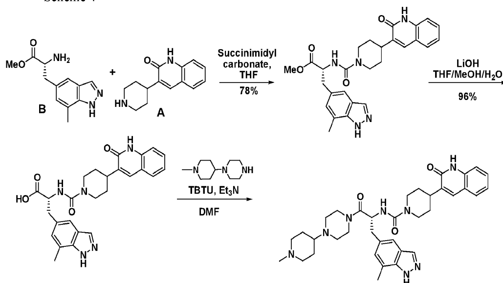
Scheme 4
