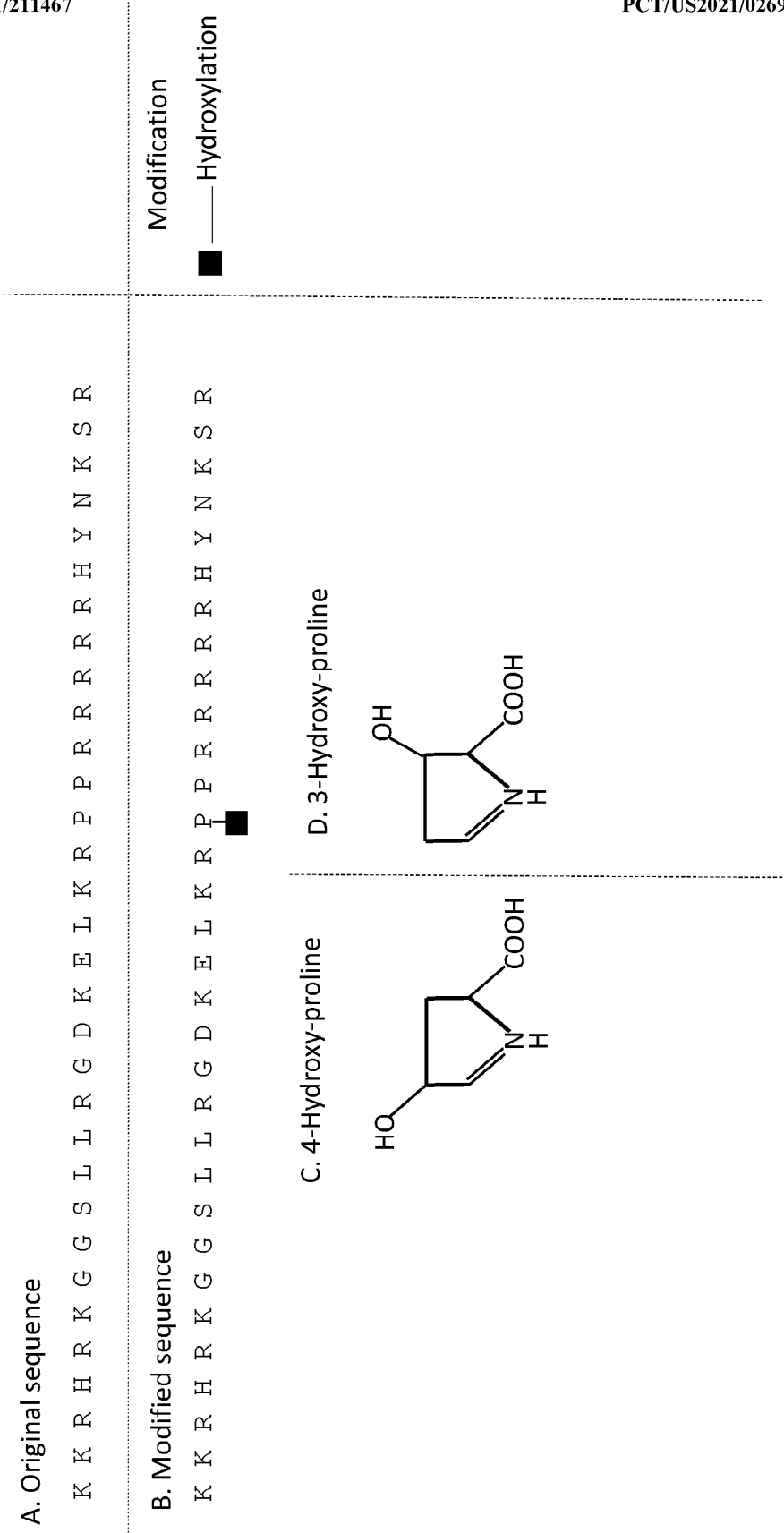
Figure 29: Hydroxylation
