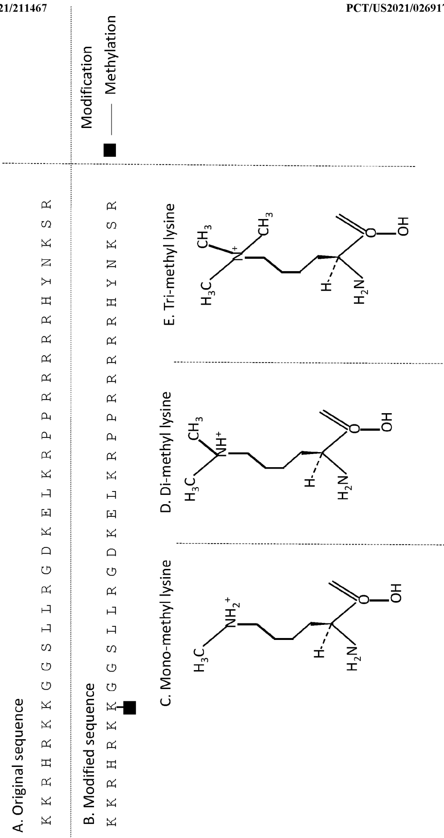
Figure 28: Methylation
