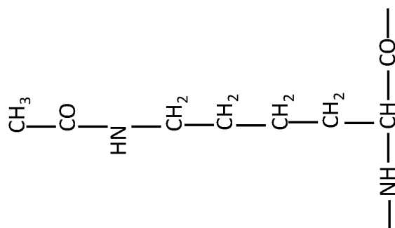
Figure 5: Acetyl-lysine
