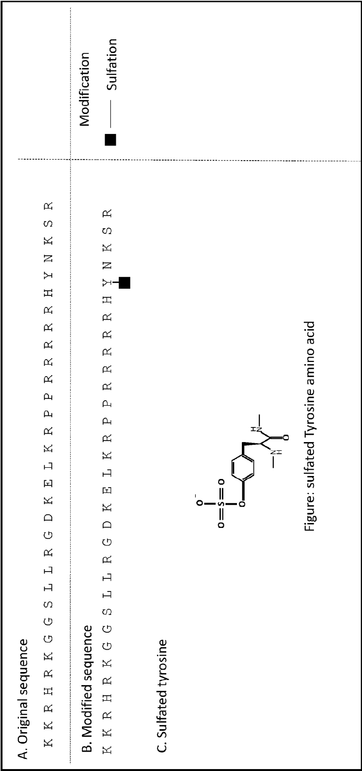
Figure 25: Sulfation
