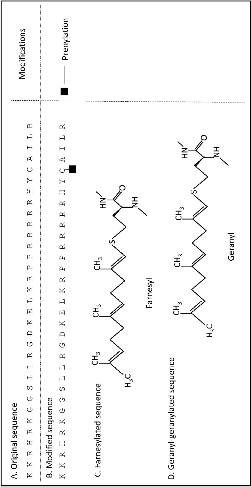
Figure 26: Prenylation
