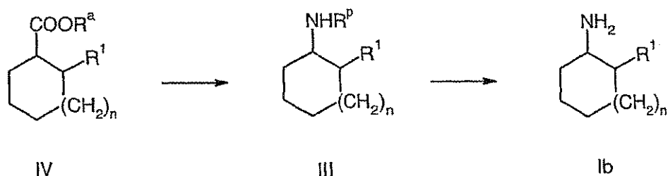
10 Scheme 2
