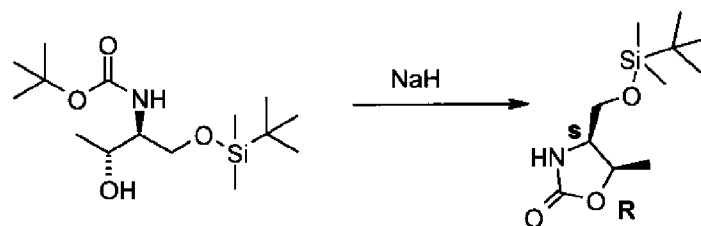
Scheme 6
