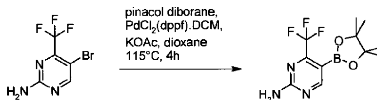
Intermediate B
