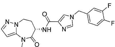
(S)-1-(3,4-difluorobenzyl)-N-(4-methyl-5-oxo-5,6,7,8-tetrahydro-4H-pyrazolo[1,5-a][1,3]diazepin-6-yl)-1H-imidazole-4-carboxamide
