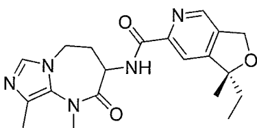
(1R)-N-(1,9-dimethyl-2-oxo-2,3,4,5-tetrahydro-1H-imidazo[1,5-a][1,3]diazepin-3-yl)-1-ethyl-1-methyl-1,3-dihydrofuro[3,4-c]pyridine-6-carboxamide
