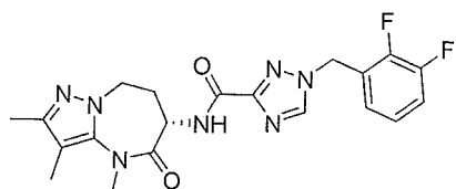
(S)-1-(2,3-difluorobenzyl)-N-(2,3,4-trimethyl-5-oxo-5,6,7,8-tetrahydro-4H-pyrazolo[1,5-a][1,3]diazepin-6-yl)-1H-1,2,4-triazole-3-carboxamide
