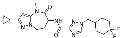
N-(2-cyclopropyl-4-methyl-5-oxo-5,6,7,8-tetrahydro-4H-pyrazolo[1,5-a][1,3]diazepin-6-yl)-1-((4,4-difluorocyclohexyl)methyl)-1H-1,2,4-triazole-3-carboxamide
