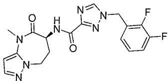
1-[(2,3-difluorophenyl)methyl]-N-[rac-(6S)-4-methyl-5-oxo-7,8-dihydro-6H-pyrazolo[1,5-a][1,3]diazepin-6-yl]-1,2,4-triazole-3-carboxamide
