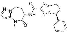
rac-(5S)-5-phenyl-N-[rac-(6S)-4-methyl-5-oxo-7,8-dihydro-6H-pyrazolo[1,5-a][1,3]diazepin-6-yl]-6,7-dihydro-5H-pyrrolo[1,2-b][1,2,4]triazole-2-carboxamide
