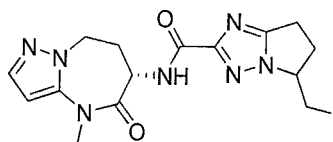
5-ethyl-N-[(6S)-4-methyl-5-oxo-7,8-dihydro-6H-pyrazolo[1,5-a][1,3]diazepin-6-yl]-6,7-dihydro-5H-pyrrolo[1,2-b][1,2,4]triazole-2-carboxamide
