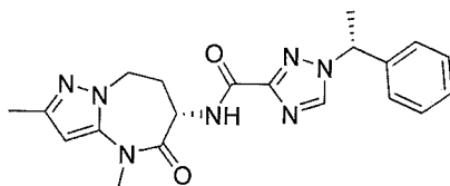
N-((S)-2,4-dimethyl-5-oxo-5,6,7,8-tetrahydro-4H-pyrazolo[1,5-a][1,3]diazepin-6-yl)-1-((R)-1-phenylethyl)-1H-1,2,4-triazole-3-carboxamide
