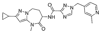
N-(2-cyclopropyl-4-methyl-5-oxo-5,6,7,8-tetrahydro-4H-pyrazolo[1,5-a][1,3]diazepin-6-yl)-1-((2-methylpyridin-4-yl)methyl)-1H-1,2,4-triazole-3-carboxamide
