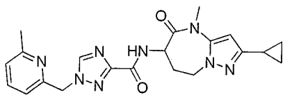
N-(2-cyclopropyl-4-methyl-5-oxo-5,6,7,8-tetrahydro-4H-pyrazolo[1,5-a][1,3]diazepin-6-yl)-1-((6-methylpyridin-2-yl)methyl)-1H-1,2,4-triazole-3-carboxamide
