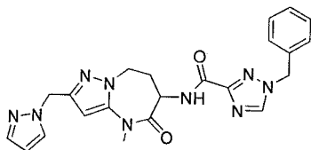
1-benzyl-N-[4-methyl-5-oxo-2-(pyrazol-1-ylmethyl)-7,8-dihydro-6H-pyrazolo[1,5-a][1,3]diazepin-6-yl]-1,2,4-triazole-3-carboxamide
