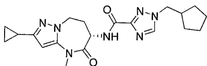
(S)-1-(cyclopentylmethyl)-N-(2-cyclopropyl-4-methyl-5-oxo-5,6,7,8-tetrahydro-4H-pyrazolo[1,5-a][1,3]diazepin-6-yl)-1H-1,2,4-triazole-3-carboxamide
