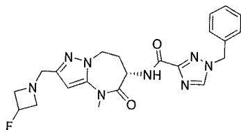
(S)-1-benzyl-N-(2-((3-fluoroazetidin-1-yl)methyl)-4-methyl-5-oxo-5,6,7,8-tetrahydro-4H-pyrazolo[1,5-a][1,3]diazepin-6-yl)-1H-1,2,4-triazole-3-carboxamide
