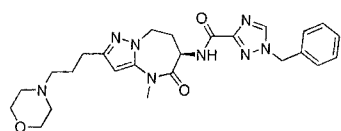
1-benzyl-N-[(6R)-4-methyl-2-(3-morpholinopropyl)-5-oxo-7,8-dihydro-6H-pyrazolo[1,5-a][1,3]diazepin-6-yl]-1,2,4-triazole-3-carboxamide
