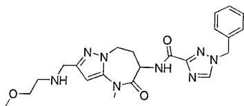
1-benzyl-N-[2-[(2-methoxyethylamino)methyl]-4-methyl-5-oxo-7,8-dihydro-6H-pyrazolo[1,5-a][1,3]diazepin-6-yl]-1,2,4-triazole-3-carboxamide
