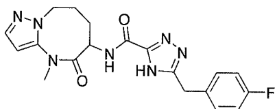
5-(4-fluorobenzyl)-N-(4-methyl-5-oxo-4,5,6,7,8,9-hexahydropyrazolo[1,5-a][1,3]diazocin-6-yl)-4H-1,2,4-triazole-3-carboxamide
