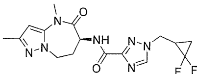
1-((2,2-difluorocyclopropyl)methyl)-N-((S)-2,4-dimethyl-5-oxo-5,6,7,8-tetrahydro-4H-pyrazolo[1,5-a][1,3]diazepin-6-yl)-1H-1,2,4-triazole-3-carboxamide
