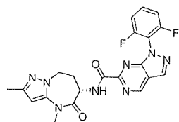
1-(2,6-difluorophenyl)-N-[(6S)-2,4-dimethyl-5-oxo-7,8-dihydro-6H-pyrazolo[1,5-a][1,3]diazepin-6-yl]pyrazolo[3,4-d]pyrimidine-6-carboxamide
