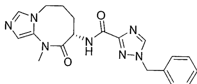
(S)-1-benzyl-N-(1-methyl-2-oxo-1,2,3,4,5,6-hexahydroimidazo[1,5-a][1,3]diazocin-3-yl)-1H-1,2,4-triazole-3-carboxamide
