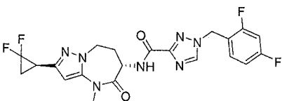
1-(2,4-difluorobenzyl)-N-((S)-2-((R)-2,2-difluorocyclopropyl)-4-methyl-5-oxo-5,6,7,8-tetrahydro-4H-pyrazolo[1,5-a][1,3]diazepin-6-yl)-1H-1,2,4-triazole-3-carboxamide
