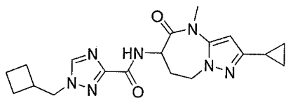
1-(cyclobutylmethyl)-N-(2-cyclopropyl-4-methyl-5-oxo-5,6,7,8-tetrahydro-4H-pyrazolo[1,5-a][1,3]diazepin-6-yl)-1H-1,2,4-triazole-3-carboxamide
