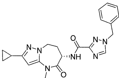
(S)-1-benzyl-N-(2-cyclopropyl-4-methyl-5-oxo-5,6,7,8-tetrahydro-4H-pyrazolo[1,5-a][1,3]diazepin-6-yl)-1H-1,2,4-triazole-3-carboxamide
