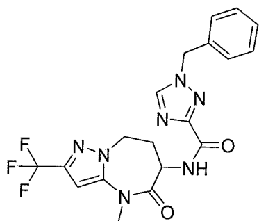
1-benzyl-N-(4-methyl-5-oxo-2-(trifluoromethyl)-5,6,7,8-tetrahydro-4H-pyrazolo[1,5-a][1,3]diazepin-6-yl)-1H-1,2,4-triazole-3-carboxamide
