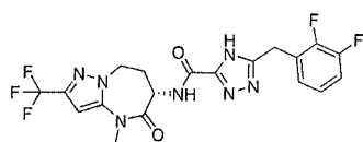
5-[(2,3-difluorophenyl)methyl]-N-(6S)-4-methyl-5-oxo-2-(trifluoromethyl)-7,8-dihydro-6H-pyrazolo[1,5-a][1,3]diazepin-6-yl-4H-1,2,4-triazole-3-carboxamide
