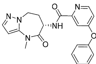
(S)-N-(4-methyl-5-oxo-5,6,7,8-tetrahydro-4H-pyrazolo[1,5-a][1,3]diazepin-6-yl)-4-phenoxycolinamide
