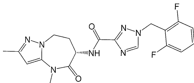
(S)-1-(2,6-difluorobenzyl)-N-(2,4-dimethyl-5-oxo-5,6,7,8-tetrahydro-4H-pyrazolo[1,5-a][1,3]diazepin-6-yl)-1H-1,2,4-triazole-3-carboxamide,
