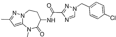
1-(4-chlorobenzyl)-N-(2,4-dimethyl-5-oxo-5,6,7,8-tetrahydro-4H-pyrazolo[1,5-a][1,3]diazepin-6-yl)-1H-1,2,4-triazole-3-carboxamide
