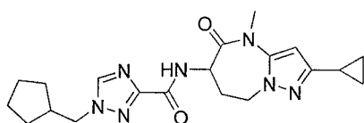
1-(cyclopentylmethyl)-N-(2-cyclopropyl-4-methyl-5-oxo-5,6,7,8-tetrahydro-4H-pyrazolo[1,5-a][1,3]diazepin-6-yl)-1H-1,2,4-triazole-3-carboxamide
