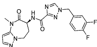
1-[(3,4-difluorophenyl)methyl]-N-[rac-(6S)-4-methyl-5-oxo-7,8-dihydro-6H-pyrazolo[1,5-a][1,3]diazepin-6-yl]-1,2,4-triazole-3-carboxamide
