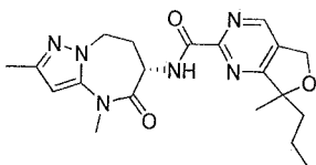
7-methyl-7-propyl-N-[(6S)-2,4-dimethyl-5-oxo-7,8-dihydro-6H-pyrazolo[1,5-a][1,3]diazepin-6-yl]-5H-furo[3,4-d]pyrimidine-2-carboxamide
