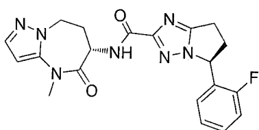
(S)-5-(2-fluorophenyl)-N-((S)-4-methyl-5-oxo-5,6,7,8-tetrahydro-4H-pyrazolo[1,5-a][1,3]diazepin-6-yl)-6,7-dihydro-5H-pyrrolo[1,2-b][1,2,4]triazole-2-carboxamide
