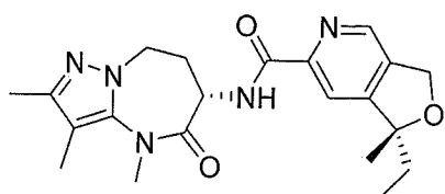
(R)-1-ethyl-1-methyl-N-((S)-2,3,4-trimethyl-5-oxo-5,6,7,8-tetrahydro-4H-pyrazolo[1,5-a][1,3]diazepin-6-yl)-1,3-dihydrofuro[3,4-c]pyridine-6-carboxamide
