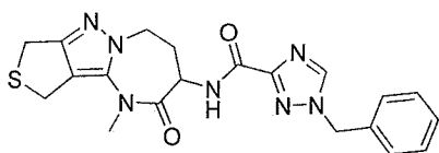
1-benzyl-N-(1-methyl-2-oxo-1,2,3,4,5,10-hexahydro-8H-thieno[3',4':3,4]pyrazolo[1,5-a][1,3]diazepin-3-yl)-1H-1,2,4-triazole-3-carboxamide
