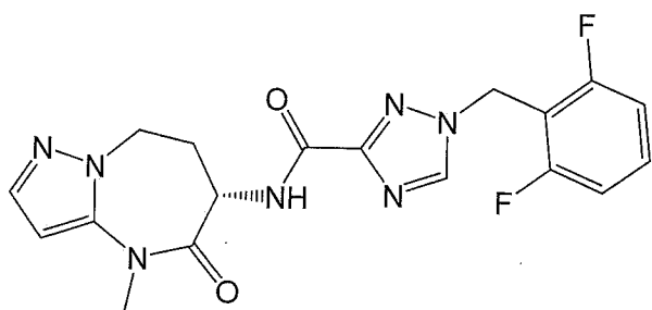
1-[(2,6-difluorophenyl)methyl]-N-[(6S)-4-methyl-5-oxo-7,8-dihydro-6H-pyrazolo[1,5-a][1,3]diazepin-6-yl]-1,2,4-triazole-3-carboxamide,
