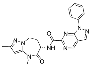
1-phenyl-N-[(6S)-2,4-dimethyl-5-oxo-7,8-dihydro-6H-pyrazolo[1,5-
