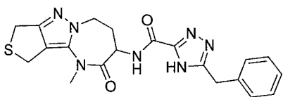
5-benzyl-N-(1-methyl-2-oxo-1,2,3,4,5,10-hexahydro-8H-thieno[3',4':3,4]pyrazolo[1,5-a][1,3]diazepin-3-yl)-4H-1,2,4-triazole-3-carboxamide
