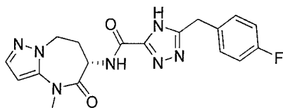
(S)-5-(4-fluorobenzyl)-N-(4-methyl-5-oxo-5,6,7,8-tetrahydro-4H-pyrazolo[1,5-a][1,3]diazepin-6-yl)-4H-1,2,4-triazole-3-carboxamide
