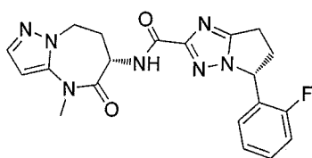
(R)-5-(2-fluorophenyl)-N-((S)-4-methyl-5-oxo-5,6,7,8-tetrahydro-4H-pyrazolo[1,5-a][1,3]diazepin-6-yl)-6,7-dihydro-5H-pyrrolo[1,2-b][1,2,4]triazole-2-carboxamide
