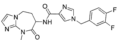
1-(3,4-difluorobenzyl)-N-(9-methyl-8-oxo-6,7,8,9-tetrahydro-5H-imidazo[1,2-a][1,3]diazepin-7-yl)-1H-imidazole-4-carboxamide
