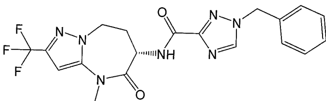
(S)-1-benzyl-N-(4-methyl-5-oxo-2-(trifluoromethyl)-5,6,7,8-tetrahydro-4H-pyrazolo[1,5-a][1,3]diazepin-6-yl)-1H-1,2,4-triazole-3-carboxamide,
