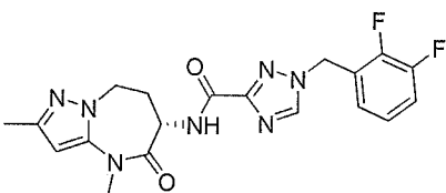
(S)-1-(2,3-difluorobenzyl)-N-(2,4-dimethyl-5-oxo-5,6,7,8-tetrahydro-4H-pyrazolo[1,5-a][1,3]diazepin-6-yl)-1H-1,2,4-triazole-3-carboxamide
