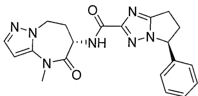
(S)-N-((S)-4-methyl-5-oxo-5,6,7,8-tetrahydro-4H-pyrazolo[1,5-a][1,3]diazepin-6-yl)-5-phenyl-6,7-dihydro-5H-pyrrolo[1,2-b][1,2,4]triazole-2-carboxamide
