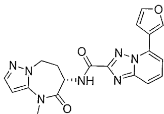
5-(3-furyl)-N-[rac-(6S)-4-methyl-5-oxo-7,8-dihydro-6H-pyrazolo[1,5-a][1,3]diazepin-6-yl]-[1,2,4]triazolo[1,5-a]pyridine-2-carboxamide
