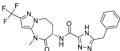
(S)-5-benzyl-N-(4-methyl-5-oxo-2-(trifluoromethyl)-5,6,7,8-tetrahydro-4H-pyrazolo[1,5-a][1,3]diazepin-6-yl)-4H-1,2,4-triazole-3-carboxamide
