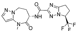
(5S)-N-[(6S)-4-methyl-5-oxo-7,8-dihydro-6H-pyrazolo[1,5-a][1,3]diazepin-6-yl]-5-(trifluoromethyl)-6,7-dihydro-5H-pyrrolo[1,2-b][1,2,4]triazole-2-carboxamide
