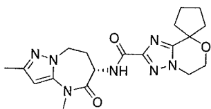
N-[(6S)-2,4-dimethyl-5-oxo-7,8-dihydro-6H-pyrazolo[1,5-a][1,3]diazepin-6-yl]spiro[5,6-dihydro-[1,2,4]triazolo[5,1-c][1,4]oxazine-8,1'-cyclopentane]-2-carboxamide
