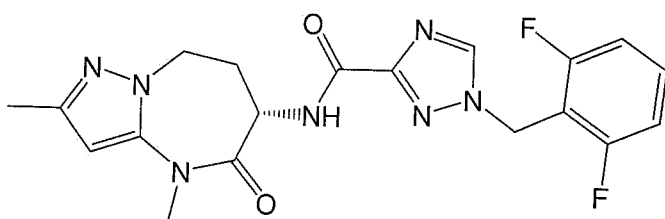
(S)-1-(2,6-difluorobenzyl)-N-(2,4-dimethyl-5-oxo-5,6,7,8-tetrahydro-4H-pyrazolo[1,5-a][1,3]diazepin-6-yl)-1H-1,2,4-triazole-3-carboxamide,
