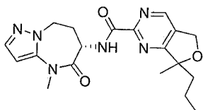
7-methyl-7-propyl-N-[(6S)-4-methyl-5-oxo-7,8-dihydro-6H-pyrazolo[1,5-a][1,3]diazepin-6-yl]-5H-furo[3,4-d]pyrimidine-2-carboxamide
