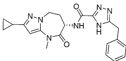
(S)-5-benzyl-N-(2-cyclopropyl-4-methyl-5-oxo-5,6,7,8-tetrahydro-4H-pyrazolo[1,5-a][1,3]diazepin-6-yl)-4H-1,2,4-triazole-3-carboxamide
