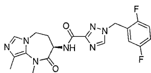
1-[(2,5-difluorophenyl)methyl]-N-(3R)-1,9-dimethyl-2-oxo-4,5-dihydro-3H-imidazo[1,5-a][1,3]diazepin-3-yl-1,2,4-triazole-3-carboxamide
