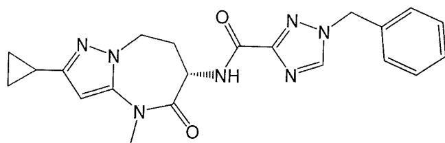
(S)-1-benzyl-N-(2-cyclopropyl-4-methyl-5-oxo-5,6,7,8-tetrahydro-4H-pyrazolo[1,5-a][1,3]diazepin-6-yl)-1H-1,2,4-triazole-3-carboxamide,
