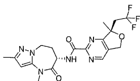
rac-(7R)-7-methyl-N-[rac-(6S)-2,4-dimethyl-5-oxo-7,8-dihydro-6H-pyrazolo[1,5-a][1,3]diazepin-6-yl]-7-(2,2,2-trifluoroethyl)-5H-furo[3,4-d]pyrimidine-2-carboxamide
