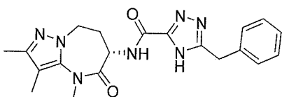
(S)-5-benzyl-N-(2,3,4-trimethyl-5-oxo-5,6,7,8-tetrahydro-4H-pyrazolo[1,5-a][1,3]diazepin-6-yl)-4H-1,2,4-triazole-3-carboxamide
