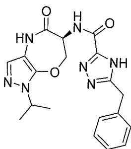
(S)-5-benzyl-N-(1-isopropyl-5-oxo-4,5,6,7-tetrahydro-1H-pyrazolo[3,4-b][1,4]oxazepin-6-yl)-4H-1,2,4-triazole-3-carboxamide
