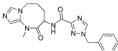
1-benzyl-N-(1-methyl-2-oxo-1,2,3,4,5,6-hexahydroimidazo[1,5-a][1,3]diazocin-3-yl)-1H-1,2,4-triazole-3-carboxamide
