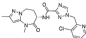
1-[(3-chloro-2-pyridyl)methyl]-N-(6S)-2,4-dimethyl-5-oxo-7,8-dihydro-6H-pyrazolo[1,5-a][1,3]diazepin-6-yl-1,2,4-triazole-3-carboxamide
