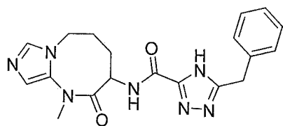
5-benzyl-N-(1-methyl-2-oxo-1,2,3,4,5,6-hexahydroimidazo[1,5-a][1,3]diazocin-3-yl)-4H-1,2,4-triazole-3-carboxamide
