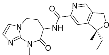
(1R)-1-ethyl-1-methyl-N-(9-methyl-8-oxo-6,7,8,9-tetrahydro-5H-imidazo[1,2-a][1,3]diazepin-7-yl)-1,3-dihydrofuro[3,4-c]pyridine-6-carboxamide
