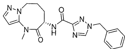
(S)-1-benzyl-N-(4-methyl-5-oxo-4,5,6,7,8,9-hexahydropyrazolo[1,5-a][1,3]diazocin-6-yl)-1H-1,2,4-triazole-3-carboxamide
