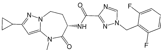
(S)-N-(2-cyclopropyl-4-methyl-5-oxo-5,6,7,8-tetrahydro-4H-pyrazolo[1,5-a][1,3]diazepin-6-yl)-1-(2,6-difluorobenzyl)-1H-1,2,4-triazole-3-carboxamide,
