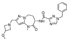
(S)-1-benzyl-N-(2-((3-methoxyazetidin-1-yl)methyl)-4-methyl-5-oxo-5,6,7,8-tetrahydro-4H-pyrazolo[1,5-a][1,3]diazepin-6-yl)-1H-1,2,4-triazole-3-carboxamide
