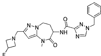
1-benzyl-N-[2-[(3-fluoroazetidin-1-yl)methyl]-4-methyl-5-oxo-7,8-dihydro-6H-pyrazolo[1,5-a][1,3]diazepin-6-yl]-1,2,4-triazole-3-carboxamide
