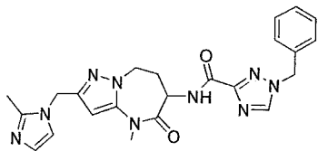
1-benzyl-N-[4-methyl-2-[(2-methylimidazol-1-yl)methyl]-5-oxo-7,8-dihydro-6H-pyrazolo[1,5-a][1,3]diazepin-6-yl]-1,2,4-triazole-3-carboxamide
