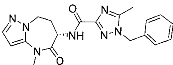
(S)-1-benzyl-5-methyl-N-(4-methyl-5-oxo-5,6,7,8-tetrahydro-4H-pyrazolo[1,5-a][1,3]diazepin-6-yl)-1H-1,2,4-triazole-3-carboxamide
