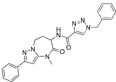
1-benzyl-N-(4-methyl-5-oxo-2-phenyl-5,6,7,8-tetrahydro-4H-pyrazolo[1,5-a][1,3]diazepin-6-yl)-1H-1,2,3-triazole-4-carboxamide
