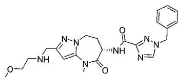
(S)-1-benzyl-N-(2-(((2-methoxyethyl)amino)methyl)-4-methyl-5-oxo-5,6,7,8-tetrahydro-4H-pyrazolo[1,5-a][1,3]diazepin-6-yl)-1H-1,2,4-triazole-3-carboxamide
