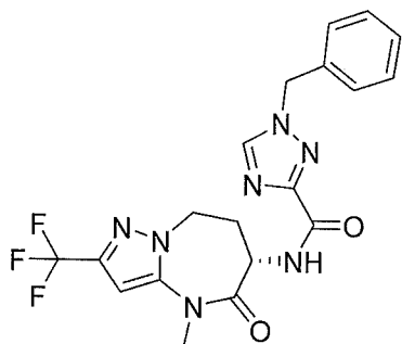
(S)-1-benzyl-N-(4-methyl-5-oxo-2-(trifluoromethyl)-5,6,7,8-tetrahydro-4H-pyrazolo[1,5-a][1,3]diazepin-6-yl)-1H-1,2,4-triazole-3-carboxamide
