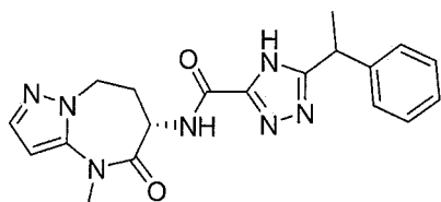
N-((S)-4-methyl-5-oxo-5,6,7,8-tetrahydro-4H-pyrazolo[1,5-a][1,3]diazepin-6-yl)-5-(1-phenylethyl)-4H-1,2,4-triazole-3-carboxamide
