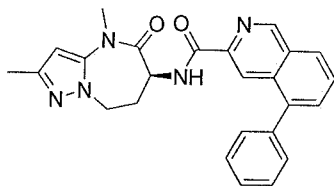
5-phenyl-N-[(6S)-2,4-dimethyl-5-oxo-7,8-dihydro-6H-pyrazolo[1,5-a][1,3]diazepin-6-yl]isoquinoline-3-carboxamide
