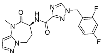
1-[(2,4-difluorophenyl)methyl]-N-[rac-(6S)-4-methyl-5-oxo-7,8-dihydro-6H-pyrazolo[1,5-a][1,3]diazepin-6-yl]-1,2,4-triazole-3-carboxamide
