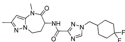
1-((4,4-difluorocyclohexyl)methyl)-N-(2,4-dimethyl-5-oxo-5,6,7,8-tetrahydro-4H-pyrazolo[1,5-a][1,3]diazepin-6-yl)-1H-1,2,4-triazole-3-carboxamide
