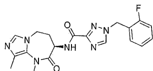
1-[(2-fluorophenyl)methyl]-N-(3R)-1,9-dimethyl-2-oxo-4,5-dihydro-3H-imidazo[1,5-a][1,3]diazepin-3-yl-1,2,4-triazole-3-carboxamide
