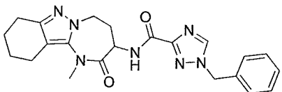
1-benzyl-N-(1-methyl-2-oxo-2,3,4,5,8,9,10,11-octahydro-1H-[1,3]diazepino[1,2-b]indazol-3-yl)-1H-1,2,4-triazole-3-carboxamide
