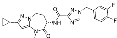
(S)-N-(2-cyclopropyl-4-methyl-5-oxo-5,6,7,8-tetrahydro-4H-pyrazolo[1,5-a][1,3]diazepin-6-yl)-1-(3,4-difluorobenzyl)-1H-1,2,4-triazole-3-carboxamide
