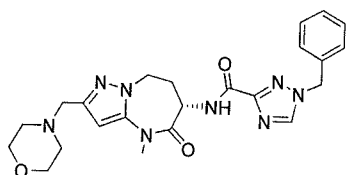
1-benzyl-N-[(6S)-4-methyl-2-(morpholinomethyl)-5-oxo-7,8-dihydro-6H-pyrazolo[1,5-a][1,3]diazepin-6-yl]-1,2,4-triazole-3-carboxamide
