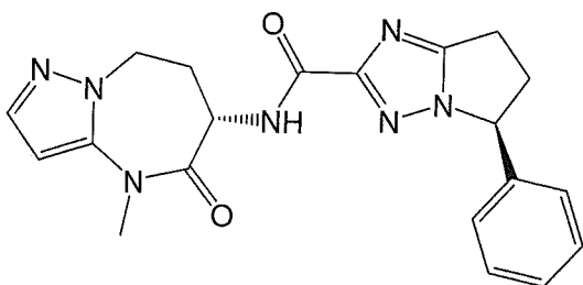
(S)-N-((S)-4-methyl-5-oxo-5,6,7,8-tetrahydro-4H-pyrazolo[1,5-a][1,3]diazepin-6-yl)-5-phenyl-6,7-dihydro-5H-pyrrolo[1,2-b][1,2,4]triazole-2-carboxamide,
