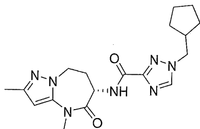
(S)-1-(cyclopentylmethyl)-N-(2,4-dimethyl-5-oxo-5,6,7,8-tetrahydro-4H-pyrazolo[1,5-a][1,3]diazepin-6-yl)-1H-1,2,4-triazole-3-carboxamide
