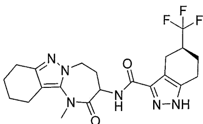
(5S)-N-(1-methyl-2-oxo-2,3,4,5,8,9,10,11-octahydro-1H-[1,3]diazepino[1,2-b]indazol-3-yl)-5-(trifluoromethyl)-4,5,6,7-tetrahydro-1H-indazole-3-carboxamide
