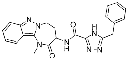
5-benzyl-N-(1-methyl-2-oxo-2,3,4,5-tetrahydro-1H-[1,3]diazepino[1,2-b]indazol-3-yl)-4H-1,2,4-triazole-3-carboxamide
