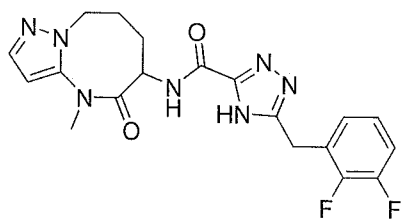
5-(2,3-difluorobenzyl)-N-(4-methyl-5-oxo-4,5,6,7,8,9-hexahydropyrazolo[1,5-a][1,3]diazocin-6-yl)-4H-1,2,4-triazole-3-carboxamide
