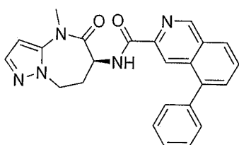
5-phenyl-N-[(6S)-4-methyl-5-oxo-7,8-dihydro-6H-pyrazolo[1,5-a][1,3]diazepin-6-yl]isoquinoline-3-carboxamide
