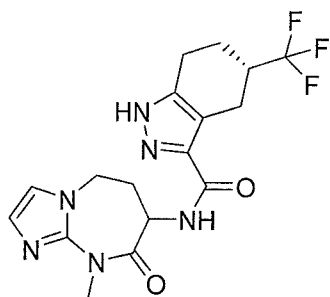
(5S)-N-(9-methyl-8-oxo-6,7,8,9-tetrahydro-5H-imidazo[1,2-a][1,3]diazepin-7-yl)-5-(trifluoromethyl)-4,5,6,7-tetrahydro-1H-indazole-3-carboxamide
