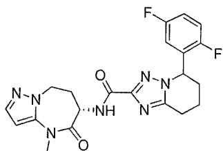
5-(2,5-difluorophenyl)-N-[rac-(6S)-4-methyl-5-oxo-7,8-dihydro-6H-pyrazolo[1,5-a][1,3]diazepin-6-yl]-5,6,7,8-tetrahydro-[1,2,4]triazolo[1,5-a]pyridine-2-carboxamide
