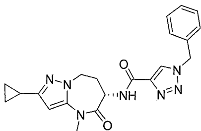
(S)-1-benzyl-N-(2-cyclopropyl-4-methyl-5-oxo-5,6,7,8-tetrahydro-4H-pyrazolo[1,5-a][1,3]diazepin-6-yl)-1H-1,2,3-triazole-4-carboxamide
