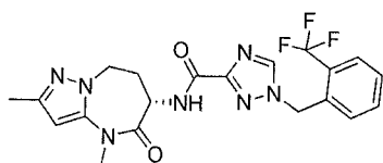
N-(6S)-2,4-dimethyl-5-oxo-7,8-dihydro-6H-pyrazolo[1,5-a][1,3]diazepin-6-yl-1-[[2-(trifluoromethyl)phenyl]methyl]-1,2,4-triazole-3-carboxamide
