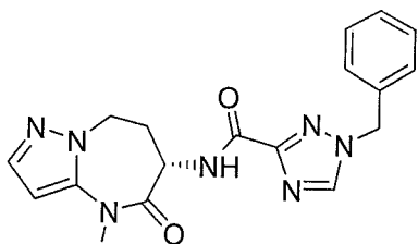
(S)-1-benzyl-N-(4-methyl-5-oxo-5,6,7,8-tetrahydro-4H-pyrazolo[1,5-a][1,3]diazepin-6-yl)-1H-1,2,4-triazole-3-carboxamide
