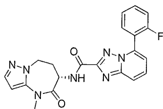
5-(2-fluorophenyl)-N-[(6S)-4-methyl-5-oxo-7,8-dihydro-6H-pyrazolo[1,5-a][1,3]diazepin-6-yl]-[1,2,4]triazolo[1,5-a]pyridine-2-carboxamide
