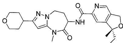
(1R)-1-ethyl-1-methyl-N-(4-methyl-5-oxo-2-(tetrahydro-2H-pyran-4-yl)-5,6,7,8-tetrahydro-4H-pyrazolo[1,5-a][1,3]diazepin-6-yl)-1,3-dihydrofuro[3,4-c]pyridine-6-carboxamide
