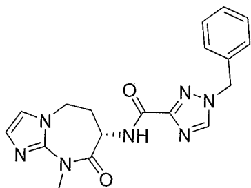
(S)-1-benzyl-N-(9-methyl-8-oxo-6,7,8,9-tetrahydro-5H-imidazo[1,2-a][1,3]diazepin-7-yl)-1H-1,2,4-triazole-3-carboxamide
