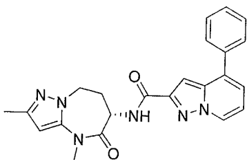
(S)-N-(2,4-dimethyl-5-oxo-5,6,7,8-tetrahydro-4H-pyrazolo[1,5-a][1,3]diazepin-6-yl)-4-phenylpyrazolo[1,5-a]pyridine-2-carboxamide
