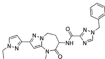
1-benzyl-N-[2-(1-ethylpyrazol-3-yl)-4-methyl-5-oxo-7,8-dihydro-6H-pyrazolo[1,5-a][1,3]diazepin-6-yl]-1,2,4-triazole-3-carboxamide
