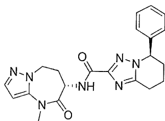
rac-(5R)-5-phenyl-N-[rac-(6S)-4-methyl-5-oxo-7,8-dihydro-6H-pyrazolo[1,5-a][1,3]diazepin-6-yl]-5,6,7,8-tetrahydro-[1,2,4]triazolo[1,5-a]pyridine-2-carboxamide
