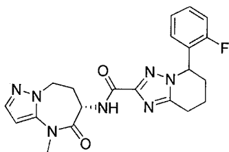
5-(2-fluorophenyl)-N-[rac-(6S)-4-methyl-5-oxo-7,8-dihydro-6H-pyrazolo[1,5-a][1,3]diazepin-6-yl]-5,6,7,8-tetrahydro-[1,2,4]triazolo[1,5-a]pyridine-2-carboxamide
