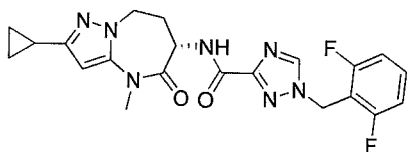
(S)-N-(2-cyclopropyl-4-methyl-5-oxo-5,6,7,8-tetrahydro-4H-pyrazolo[1,5-a][1,3]diazepin-6-yl)-1-(2,6-difluorobenzyl)-1H-1,2,4-triazole-3-carboxamide
