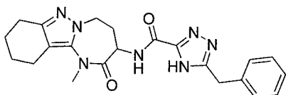
5-benzyl-N-(1-methyl-2-oxo-2,3,4,5,8,9,10,11-octahydro-1H-[1,3]diazepino[1,2-b]indazol-3-yl)-4H-1,2,4-triazole-3-carboxamide
