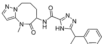
N-(4-methyl-5-oxo-4,5,6,7,8,9-hexahydropyrazolo[1,5-a][1,3]diazocin-6-yl)-5-(1-phenylethyl)-4H-1,2,4-triazole-3-carboxamide
