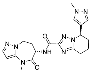
rac-(5R)-5-(1-methylpyrazol-4-yl)-N-[rac-(6S)-4-methyl-5-oxo-7,8-dihydro-6H-pyrazolo[1,5-a][1,3]diazepin-6-yl]-5,6,7,8-tetrahydro-[1,2,4]triazolo[1,5-a]pyridine-2-carboxamide
