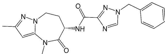
(S)-1-benzyl-N-(2,4-dimethyl-5-oxo-5,6,7,8-tetrahydro-4H-pyrazolo[1,5-a][1,3]diazepin-6-yl)-1H-1,2,4-triazole-3-carboxamide,
