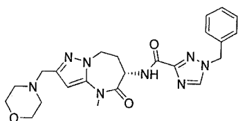
1-benzyl-N-[(6S)-4-methyl-2-(morpholinomethyl)-5-oxo-7,8-dihydro-6H-pyrazolo[1,5-a][1,3]diazepin-6-yl]-1,2,4-triazole-3-carboxamide
