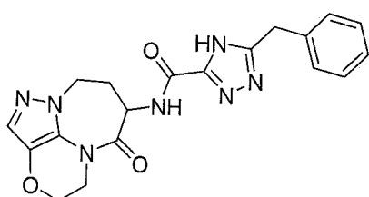
5-benzyl-N-(6-oxo-4,5,6,7,8,9-hexahydro-3-oxa-1,5a,9a-triazabenzocd]azulen-7-yl)-1H-1,2,4-triazole-3-carboxamide
