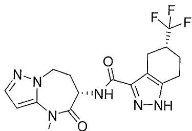
(R)-N-((S)-4-methyl-5-oxo-5,6,7,8-tetrahydro-4H-pyrazolo[1,5-a][1,3]diazepin-6-yl)-5-(trifluoromethyl)-4,5,6,7-tetrahydro-1H-indazole-3-carboxamide
