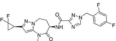
1-(2,4-difluorobenzyl)-N-((R)-2-((R)-2,2-difluorocyclopropyl)-4-methyl-5-oxo-5,6,7,8-tetrahydro-4H-pyrazolo[1,5-a][1,3]diazepin-6-yl)-1H-1,2,4-triazole-3-carboxamide
