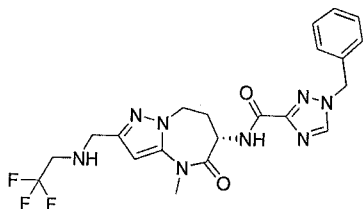
1-benzyl-N-[(6S)-4-methyl-5-oxo-2-[(2,2,2-trifluoroethylamino)methyl]-7,8-dihydro-6H-pyrazolo[1,5-a][1,3]diazepin-6-yl]-1,2,4-triazole-3-carboxamide
