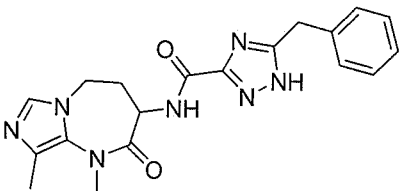
5-benzyl-N-(1,9-dimethyl-2-oxo-2,3,4,5-tetrahydro-1H-imidazo[1,5-a][1,3]diazepin-3-yl)-1H-1,2,4-triazole-3-carboxamide
