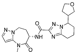
N-[(6S)-4-methyl-5-oxo-7,8-dihydro-6H-pyrazolo[1,5-a][1,3]diazepin-6-yl]-5-tetrahydrofuran-3-yl-5,6,7,8-tetrahydro-[1,2,4]triazolo[1,5-a]pyridine-2-carboxamide
