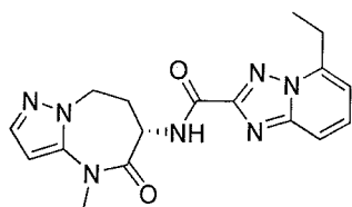
5-ethyl-N-[rac-(6S)-4-methyl-5-oxo-7,8-dihydro-6H-pyrazolo[1,5-a][1,3]diazepin-6-yl]-[1,2,4]triazolo[1,5-a]pyridine-2-carboxamide
