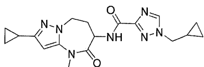
N-(2-cyclopropyl-4-methyl-5-oxo-5,6,7,8-tetrahydro-4H-pyrazolo[1,5-a][1,3]diazepin-6-yl)-1-(cyclopropylmethyl)-1H-1,2,4-triazole-3-carboxamide
