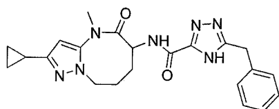
5-benzyl-N-(2-cyclopropyl-4-methyl-5-oxo-4,5,6,7,8,9-hexahydropyrazolo[1,5-a][1,3]diazocin-6-yl)-4H-1,2,4-triazole-3-carboxamide
