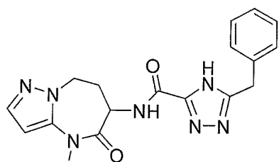
5-benzyl-N-(4-methyl-5-oxo-5,6,7,8-tetrahydro-4H-pyrazolo[1,5-a][1,3]diazepin-6-yl)-4H-1,2,4-triazole-3-carboxamide
