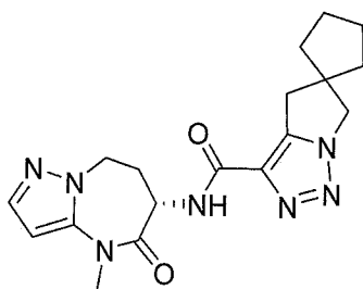
(S)-N-(4-methyl-5-oxo-5,6,7,8-tetrahydro-4H-pyrazolo[1,5-a][1,3]diazepin-6-yl)-4'H,6'H-spiro[cyclopentane-1,5'-pyrrolo[1,2-c][1,2,3]triazole]-3'-carboxamide
