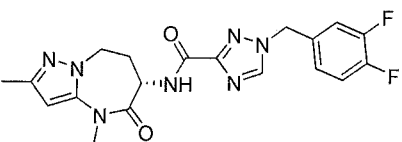
(S)-1-(3,4-difluorobenzyl)-N-(2,4-dimethyl-5-oxo-5,6,7,8-tetrahydro-4H-pyrazolo[1,5-a][1,3]diazepin-6-yl)-1H-1,2,4-triazole-3-carboxamide
