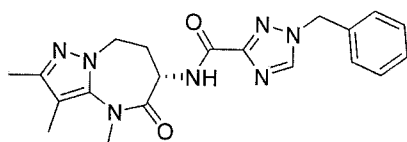
(S)-1-benzyl-N-(2,3,4-trimethyl-5-oxo-5,6,7,8-tetrahydro-4H-pyrazolo[1,5-a][1,3]diazepin-6-yl)-1H-1,2,4-triazole-3-carboxamide
