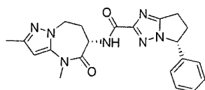
(5R)-5-phenyl-N-[(6S)-2,4-dimethyl-5-oxo-7,8-dihydro-6H-pyrazolo[1,5-a][1,3]diazepin-6-yl]-6,7-dihydro-5H-pyrrolo[1,2-b][1,2,4]triazole-2-carboxamide
