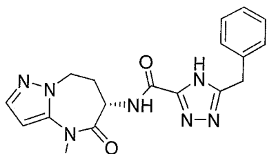
(S)-5-benzyl-N-(4-methyl-5-oxo-5,6,7,8-tetrahydro-4H-pyrazolo[1,5-a][1,3]diazepin-6-yl)-4H-1,2,4-triazole-3-carboxamide
