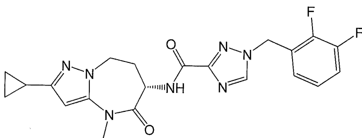
(S)-N-(2-cyclopropyl-4-methyl-5-oxo-5,6,7,8-tetrahydro-4H-pyrazolo[1,5-a][1,3]diazepin-6-yl)-1-(2,3-difluorobenzyl)-1H-1,2,4-triazole-3-carboxamide,
