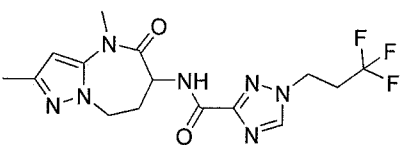
N-(2,4-dimethyl-5-oxo-5,6,7,8-tetrahydro-4H-pyrazolo[1,5-a][1,3]diazepin-6-yl)-1-(3,3,3-trifluoropropyl)-1H-1,2,4-triazole-3-carboxamide
