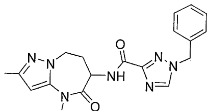
1-benzyl-N-(2,4-dimethyl-5-oxo-5,6,7,8-tetrahydro-4H-pyrazolo[1,5-a][1,3]diazepin-6-yl)-1H-1,2,4-triazole-3-carboxamide
