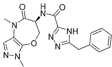
(S)-5-benzyl-N-(1,4-dimethyl-5-oxo-4,5,6,7-tetrahydro-1H-pyrazolo[3,4-b][1,4]oxazepin-6-yl)-4H-1,2,4-triazole-3-carboxamide
