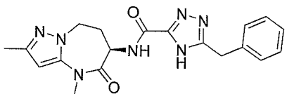
(R)-5-benzyl-N-(2,4-dimethyl-5-oxo-5,6,7,8-tetrahydro-4H-pyrazolo[1,5-a][1,3]diazepin-6-yl)-4H-1,2,4-triazole-3-carboxamide
