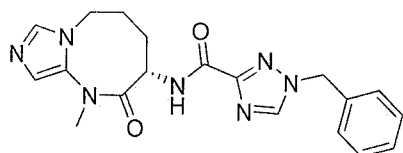
(S)-1-benzyl-N-(1-methyl-2-oxo-1,2,3,4,5,6-hexahydroimidazo[1,5-a][1,3]diazocin-3-yl)-1H-1,2,4-triazole-3-carboxamide
