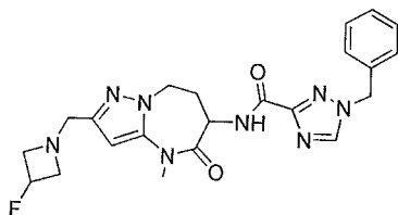
1-benzyl-N-[2-[(3-fluoroazetidin-1-yl)methyl]-4-methyl-5-oxo-7,8-dihydro-6H-pyrazolo[1,5-a][1,3]diazepin-6-yl]-1,2,4-triazole-3-carboxamide
