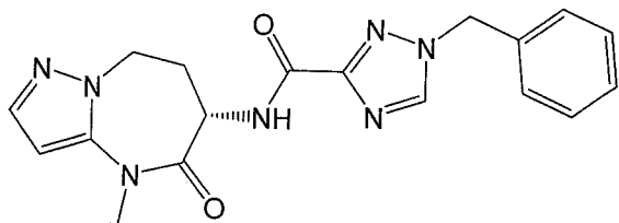
(S)-1-benzyl-N-(4-methyl-5-oxo-5,6,7,8-tetrahydro-4H-pyrazolo[1,5-a][1,3]diazepin-6-yl)-1H-1,2,4-triazole-3-carboxamide,
