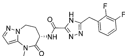
(S)-5-(2,3-difluorobenzyl)-N-(4-methyl-5-oxo-5,6,7,8-tetrahydro-4H-pyrazolo[1,5-a][1,3]diazepin-6-yl)-4H-1,2,4-triazole-3-carboxamide
