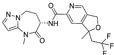
1-methyl-N-((S)-4-methyl-5-oxo-5,6,7,8-tetrahydro-4H-pyrazolo[1,5-a][1,3]diazepin-6-yl)-1-(2,2,2-trifluoroethyl)-1,3-dihydrofuro[3,4-c]pyridine-6-carboxamide
