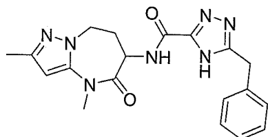
5-benzyl-N-(2,4-dimethyl-5-oxo-5,6,7,8-tetrahydro-4H-pyrazolo[1,5-a][1,3]diazepin-6-yl)-4H-1,2,4-triazole-3-carboxamide
