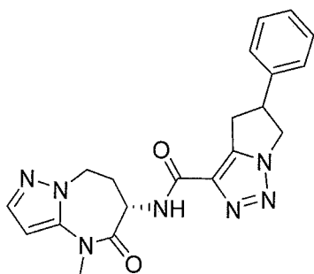
N-((S)-4-methyl-5-oxo-5,6,7,8-tetrahydro-4H-pyrazolo[1,5-a][1,3]diazepin-6-yl)-5-phenyl-5,6-dihydro-4H-pyrrolo[1,2-c][1,2,3]triazole-3-carboxamide
