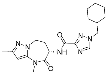
(S)-1-(cyclohexylmethyl)-N-(2,4-dimethyl-5-oxo-5,6,7,8-tetrahydro-4H-pyrazolo[1,5-a][1,3]diazepin-6-yl)-1H-1,2,4-triazole-3-carboxamide
