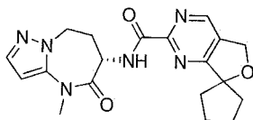
N-[rac-(6S)-4-methyl-5-oxo-7,8-dihydro-6H-pyrazolo[1,5-a][1,3]diazepin-6-yl]spiro[5H-furo[3,4-d]pyrimidine-7,1'-cyclopentane]-2-carboxamide
