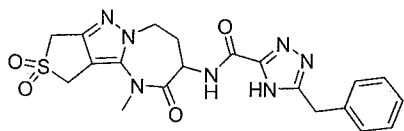
5-benzyl-N-(1-methyl-9,9-dioxido-2-oxo-1,2,3,4,5,10-hexahydro-8H-thieno[3',4':3,4]pyrazolo[1,5-a][1,3]diazepin-3-yl)-4H-1,2,4-triazole-3-carboxamide
