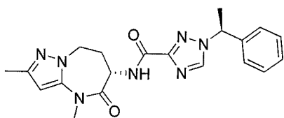
N-((S)-2,4-dimethyl-5-oxo-5,6,7,8-tetrahydro-4H-pyrazolo[1,5-a][1,3]diazepin-6-yl)-1-((S)-1-phenylethyl)-1H-1,2,4-triazole-3-carboxamide
