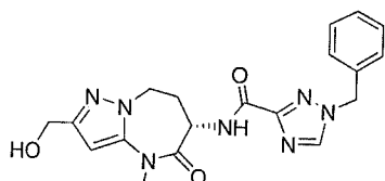
1-benzyl-N-[(6S)-2-(hydroxymethyl)-4-methyl-5-oxo-7,8-dihydro-6H-pyrazolo[1,5-a][1,3]diazepin-6-yl]-1H-1,2,4-triazole-3-carboxamide
