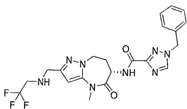
1-benzyl-N-[(6S)-4-methyl-5-oxo-2-[(2,2,2-trifluoroethylamino)methyl]-7,8-dihydro-6H-pyrazolo[1,5-a][1,3]diazepin-6-yl]-1,2,4-triazole-3-carboxamide
