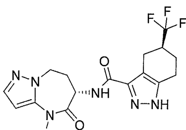
(S)-N-((S)-4-methyl-5-oxo-5,6,7,8-tetrahydro-4H-pyrazolo[1,5-a][1,3]diazepin-6-yl)-5-(trifluoromethyl)-4,5,6,7-tetrahydro-1H-indazole-3-carboxamide
