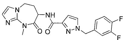
1-(3,4-difluorobenzyl)-N-(9-methyl-8-oxo-6,7,8,9-tetrahydro-5H-imidazo[1,2-a][1,3]diazepin-7-yl)-1H-pyrazole-3-carboxamide
