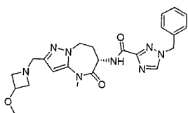
(S)-1-benzyl-N-(2-((3-methoxyazetidin-1-yl)methyl)-4-methyl-5-oxo-5,6,7,8-tetrahydro-4H-pyrazolo[1,5-a][1,3]diazepin-6-yl)-1H-1,2,4-triazole-3-carboxamide
