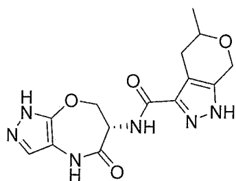
5-methyl-N-((S)-5-oxo-4,5,6,7-tetrahydro-1H-pyrazolo[3,4-b][1,4]oxazepin-6-yl)-1,4,5,7-tetrahydropyrano[3,4-c]pyrazole-3-carboxamide
