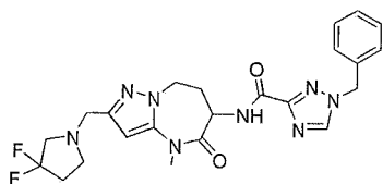
1-benzyl-N-[2-[(3,3-difluoropyrrolidin-1-yl)methyl]-4-methyl-5-oxo-7,8-dihydro-6H-pyrazolo[1,5-a][1,3]diazepin-6-yl]-1,2,4-triazole-3-carboxamide
