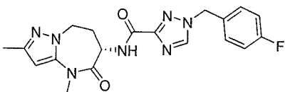
(S)-N-(2,4-dimethyl-5-oxo-5,6,7,8-tetrahydro-4H-pyrazolo[1,5-a][1,3]diazepin-6-yl)-1-(4-fluorobenzyl)-1H-1,2,4-triazole-3-carboxamide
