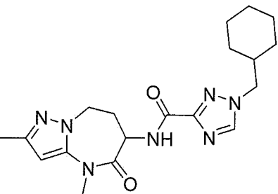
1-(cyclohexylmethyl)-N-(2,4-dimethyl-5-oxo-5,6,7,8-tetrahydro-4H-pyrazolo[1,5-a][1,3]diazepin-6-yl)-1H-1,2,4-triazole-3-carboxamide
