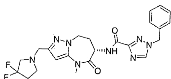
(S)-1-benzyl-N-(2-((3,3-difluoropyrrolidin-1-yl)methyl)-4-methyl-5-oxo-5,6,7,8-tetrahydro-4H-pyrazolo[1,5-a][1,3]diazepin-6-yl)-1H-1,2,4-triazole-3-carboxamide
