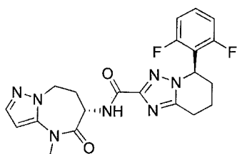
rac-(5R)-5-(2,6-difluorophenyl)-N-[rac-(6S)-4-methyl-5-oxo-7,8-dihydro-6H-pyrazolo[1,5-a][1,3]diazepin-6-yl]-5,6,7,8-tetrahydro-[1,2,4]triazolo[1,5-a]pyridine-2-carboxamide
