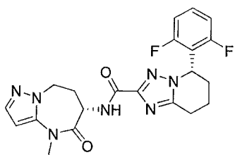
rac-(5S)-5-(2,6-difluorophenyl)-N-[rac-(6S)-4-methyl-5-oxo-7,8-dihydro-6H-pyrazolo[1,5-a][1,3]diazepin-6-yl]-5,6,7,8-tetrahydro-[1,2,4]triazolo[1,5-a]pyridine-2-carboxamide
