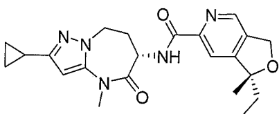
(R)-N-((S)-2-cyclopropyl-4-methyl-5-oxo-5,6,7,8-tetrahydro-4H-pyrazolo[1,5-a][1,3]diazepin-6-yl)-1-ethyl-1-methyl-1,3-dihydrofuro[3,4-c]pyridine-6-carboxamide
