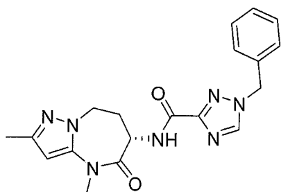
(S)-1-benzyl-N-(2,4-dimethyl-5-oxo-5,6,7,8-tetrahydro-4H-pyrazolo[1,5-a][1,3]diazepin-6-yl)-1H-1,2,4-triazole-3-carboxamide
