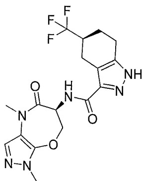
(S)-N-((S)-1,4-dimethyl-5-oxo-4,5,6,7-tetrahydro-1H-pyrazolo[3,4-b][1,4]oxazepin-6-yl)-5-(trifluoromethyl)-4,5,6,7-tetrahydro-1H-indazole-3-carboxamide
