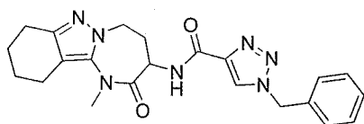
1-benzyl-N-(1-methyl-2-oxo-2,3,4,5,8,9,10,11-octahydro-1H-[1,3]diazepino[1,2-b]indazol-3-yl)-1H-1,2,3-triazole-4-carboxamide
