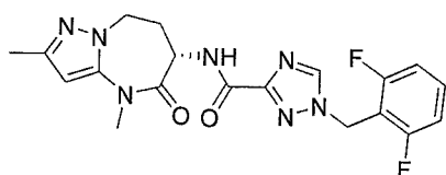
(S)-1-(2,6-difluorobenzyl)-N-(2,4-dimethyl-5-oxo-5,6,7,8-tetrahydro-4H-pyrazolo[1,5-a][1,3]diazepin-6-yl)-1H-1,2,4-triazole-3-carboxamide
