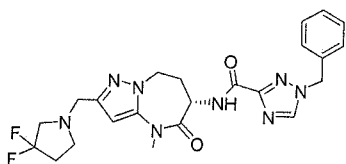
(S)-1-benzyl-N-(2-((3,3-difluoropyrrolidin-1-yl)methyl)-4-methyl-5-oxo-5,6,7,8-tetrahydro-4H-pyrazolo[1,5-a][1,3]diazepin-6-yl)-1H-1,2,4-triazole-3-carboxamide
