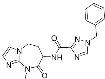
1-benzyl-N-(9-methyl-8-oxo-6,7,8,9-tetrahydro-5H-imidazo[1,2-a][1,3]diazepin-7-yl)-1H-1,2,4-triazole-3-carboxamide
