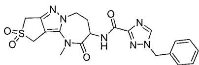
1-benzyl-N-(1-methyl-9,9-dioxido-2-oxo-1,2,3,4,5,10-hexahydro-8H-thieno[3',4':3,4]pyrazolo[1,5-a][1,3]diazepin-3-yl)-1H-1,2,4-triazole-3-carboxamide
