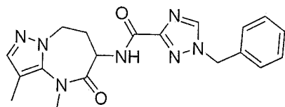
1-benzyl-N-(3,4-dimethyl-5-oxo-5,6,7,8-tetrahydro-4H-pyrazolo[1,5-a][1,3]diazepin-6-yl)-1H-1,2,4-triazole-3-carboxamide
