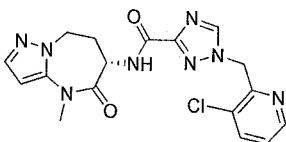
1-[(3-chloro-2-pyridyl)methyl]-N-(6S)-4-methyl-5-oxo-7,8-dihydro-6H-pyrazolo[1,5-a][1,3]diazepin-6-yl-1,2,4-triazole-3-carboxamide
