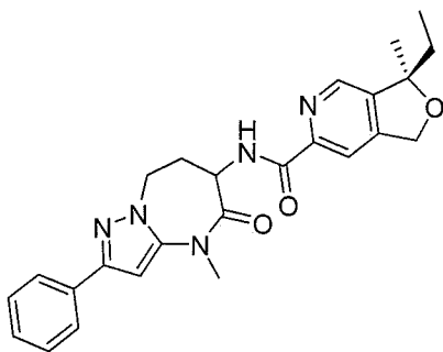
(3R)-3-ethyl-3-methyl-N-(4-methyl-5-oxo-2-phenyl-5,6,7,8-tetrahydro-4H-pyrazolo[1,5-a][1,3]diazepin-6-yl)-1,3-dihydrofuro[3,4-c]pyridine-6-carboxamide
