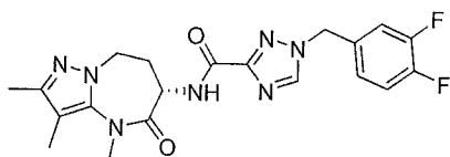
(S)-1-(3,4-difluorobenzyl)-N-(2,3,4-trimethyl-5-oxo-5,6,7,8-tetrahydro-4H-pyrazolo[1,5-a][1,3]diazepin-6-yl)-1H-1,2,4-triazole-3-carboxamide
