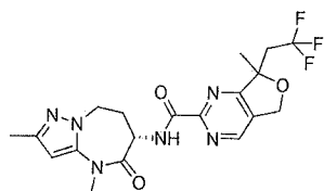
7-methyl-N-[(6S)-2,4-dimethyl-5-oxo-7,8-dihydro-6H-pyrazolo[1,5-a][1,3]diazepin-6-yl]-7-(2,2,2-trifluoroethyl)-5H-furo[3,4-d]pyrimidine-2-carboxamide
