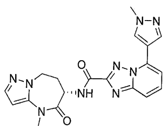
N-[(6S)-4-methyl-5-oxo-7,8-dihydro-6H-pyrazolo[1,5-a][1,3]diazepin-6-yl]-5-(1-methylpyrazol-4-yl)-[1,2,4]triazolo[1,5-a]pyridine-2-carboxamide
