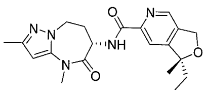
(R)-N-((S)-2,4-dimethyl-5-oxo-5,6,7,8-tetrahydro-4H-pyrazolo[1,5-a][1,3]diazepin-6-yl)-1-ethyl-1-methyl-1,3-dihydrofuro[3,4-c]pyridine-6-carboxamide
