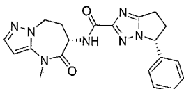
(5R)-5-phenyl-N-[(6S)-4-methyl-5-oxo-7,8-dihydro-6H-pyrazolo[1,5-a][1,3]diazepin-6-yl]-6,7-dihydro-5H-pyrrolo[1,2-b][1,2,4]triazole-2-carboxamide
