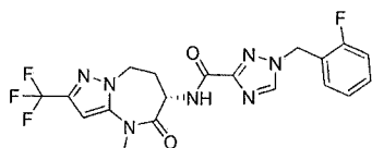
1-[(2-fluorophenyl)methyl]-N-(6S)-4-methyl-5-oxo-2-(trifluoromethyl)-7,8-dihydro-6H-pyrazolo[1,5-a][1,3]diazepin-6-yl-1,2,4-triazole-3-carboxamide
