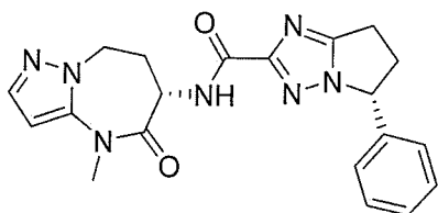
(R)-N-((S)-4-methyl-5-oxo-5,6,7,8-tetrahydro-4H-pyrazolo[1,5-a][1,3]diazepin-6-yl)-5-phenyl-6,7-dihydro-5H-pyrrolo[1,2-b][1,2,4]triazole-2-carboxamide
