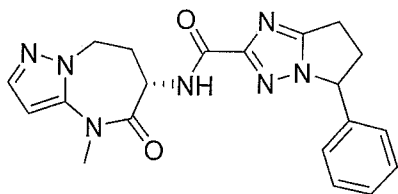
N-((S)-4-methyl-5-oxo-5,6,7,8-tetrahydro-4H-pyrazolo[1,5-a][1,3]diazepin-6-yl)-5-phenyl-6,7-dihydro-5H-pyrrolo[1,2-b][1,2,4]triazole-2-carboxamide
