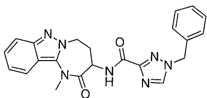
1-benzyl-N-(1-methyl-2-oxo-2,3,4,5-tetrahydro-1H-[1,3]diazepino[1,2-b]indazol-3-yl)-1H-1,2,4-triazole-3-carboxamide
