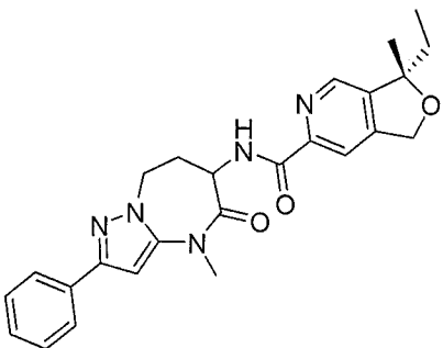
(3R)-3-ethyl-3-methyl-N-(4-methyl-5-oxo-2-phenyl-5,6,7,8-tetrahydro-4H-pyrazolo[1,5-a][1,3]diazepin-6-yl)-1,3-dihydrofuro[3,4-c]pyridine-6-carboxamide
