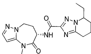
5-ethyl-N-[(6S)-4-methyl-5-oxo-7,8-dihydro-6H-pyrazolo[1,5-a][1,3]diazepin-6-yl]-5,6,7,8-tetrahydro-[1,2,4]triazolo[1,5-a]pyridine-2-
