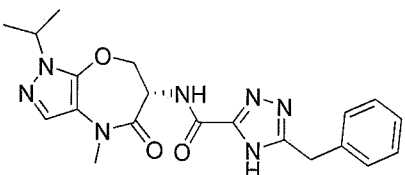
(S)-5-benzyl-N-(1-isopropyl-4-methyl-5-oxo-4,5,6,7-tetrahydro-1H-pyrazolo[3,4-b][1,4]oxazepin-6-yl)-4H-1,2,4-triazole-3-carboxamide
