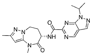
1-isopropyl-N-[(6S)-2,4-dimethyl-5-oxo-7,8-dihydro-6H-pyrazolo[1,5-a][1,3]diazepin-6-yl]pyrazolo[3,4-d]pyrimidine-6-carboxamide
