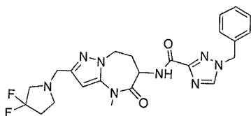
1-benzyl-N-[2-[(3,3-difluoropyrrolidin-1-yl)methyl]-4-methyl-5-oxo-7,8-dihydro-6H-pyrazolo[1,5-a][1,3]diazepin-6-yl]-1,2,4-triazole-3-carboxamide
