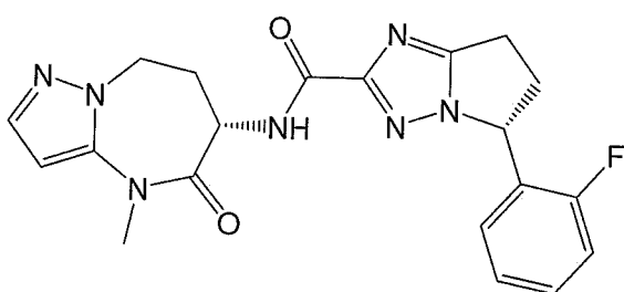
(R)-5-(2-fluorophenyl)-N-((S)-4-methyl-5-oxo-5,6,7,8-tetrahydro-4H-pyrazolo[1,5-a][1,3]diazepin-6-yl)-6,7-dihydro-5H-pyrrolo[1,2-b][1,2,4]triazole-2-carboxamide,
