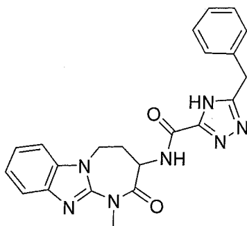
5-benzyl-N-(1-methyl-2-oxo-2,3,4,5-tetrahydro-1H-benzo[4,5]imidazo[1,2-a][1,3]diazepin-3-yl)-4H-1,2,4-triazole-3-carboxamide
