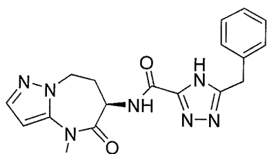
(R)-5-benzyl-N-(4-methyl-5-oxo-5,6,7,8-tetrahydro-4H-pyrazolo[1,5-a][1,3]diazepin-6-yl)-4H-1,2,4-triazole-3-carboxamide
