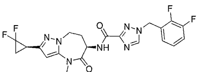
1-(2,3-difluorobenzyl)-N-((R)-2-((R)-2,2-difluorocyclopropyl)-4-methyl-5-oxo-5,6,7,8-tetrahydro-4H-pyrazolo[1,5-a][1,3]diazepin-6-yl)-1H-1,2,4-triazole-3-carboxamide
