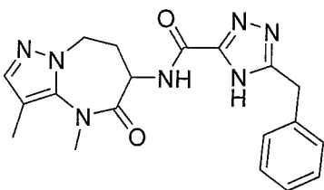
5-benzyl-N-(3,4-dimethyl-5-oxo-5,6,7,8-tetrahydro-4H-pyrazolo[1,5-a][1,3]diazepin-6-yl)-4H-1,2,4-triazole-3-carboxamide
