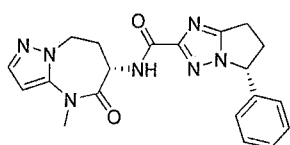
(5R)-N-[(6S)-4-methyl-5-oxo-7,8-dihydro-6H-pyrazolo[1,5-a][1,3]diazepin-
