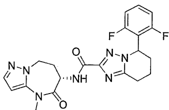
5-(2,6-difluorophenyl)-N-[rac-(6S)-4-methyl-5-oxo-7,8-dihydro-6H-pyrazolo[1,5-a][1,3]diazepin-6-yl]-5,6,7,8-tetrahydro-[1,2,4]triazolo[1,5-a]pyridine-2-carboxamide
