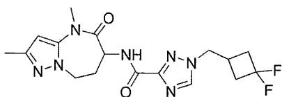
1-((3,3-difluorocyclobutyl)methyl)-N-(2,4-dimethyl-5-oxo-5,6,7,8-tetrahydro-4H-pyrazolo[1,5-a][1,3]diazepin-6-yl)-1H-1,2,4-triazole-3-carboxamide
