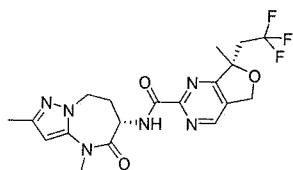
rac-(7S)-7-methyl-N-[rac-(6S)-2,4-dimethyl-5-oxo-7,8-dihydro-6H-pyrazolo[1,5-a][1,3]diazepin-6-yl]-7-(2,2,2-trifluoroethyl)-5H-furo[3,4-d]pyrimidine-2-carboxamide
