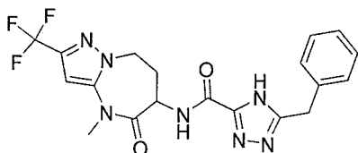
5-benzyl-N-(4-methyl-5-oxo-2-(trifluoromethyl)-5,6,7,8-tetrahydro-4H-pyrazolo[1,5-a][1,3]diazepin-6-yl)-4H-1,2,4-triazole-3-carboxamide
