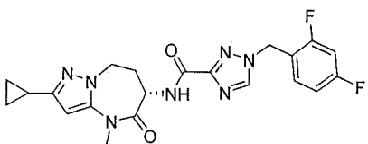
(S)-N-(2-cyclopropyl-4-methyl-5-oxo-5,6,7,8-tetrahydro-4H-pyrazolo[1,5-a][1,3]diazepin-6-yl)-1-(2,4-difluorobenzyl)-1H-1,2,4-triazole-3-carboxamide
