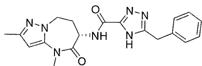
(S)-5-benzyl-N-(2,4-dimethyl-5-oxo-5,6,7,8-tetrahydro-4H-pyrazolo[1,5-a][1,3]diazepin-6-yl)-4H-1,2,4-triazole-3-carboxamide
