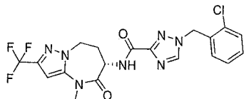
1-[(2-chlorophenyl)methyl]-N-(6S)-4-methyl-5-oxo-2-(trifluoromethyl)-7,8-dihydro-6H-pyrazolo[1,5-a][1,3]diazepin-6-yl-1,2,4-triazole-3-carboxamide
