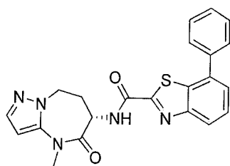
7-phenyl-N-[rac-(6S)-4-methyl-5-oxo-7,8-dihydro-6H-pyrazolo[1,5-a][1,3]diazepin-6-yl]-1,3-benzothiazole-2-carboxamide
