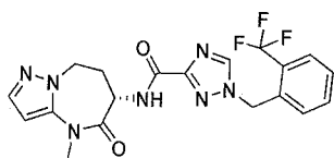
N-(6S)-4-methyl-5-oxo-7,8-dihydro-6H-pyrazolo[1,5-a][1,3]diazepin-6-yl-1-[[2-(trifluoromethyl)phenyl]methyl]-1,2,4-triazole-3-carboxamide
