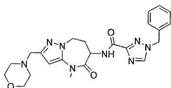
1-benzyl-N-[4-methyl-2-(morpholinomethyl)-5-oxo-7,8-dihydro-6H-pyrazolo[1,5-a][1,3]diazepin-6-yl]-1,2,4-triazole-3-carboxamide
