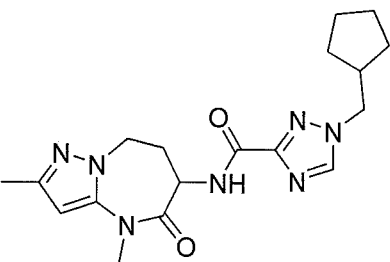
1-(cyclopentylmethyl)-N-(2,4-dimethyl-5-oxo-5,6,7,8-tetrahydro-4H-pyrazolo[1,5-a][1,3]diazepin-6-yl)-1H-1,2,4-triazole-3-carboxamide
