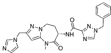
(S)-1-benzyl-N-[2-(imidazol-1-ylmethyl)-4-methyl-5-oxo-7,8-dihydro-6H-pyrazolo[1,5-a][1,3]diazepin-6-yl]-1,2,4-triazole-3-carboxamide
