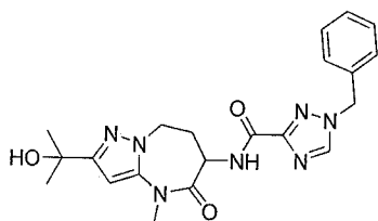
1-benzyl-N-[2-(1-hydroxy-1-methyl-ethyl)-4-methyl-5-oxo-7,8-dihydro-6H-pyrazolo[1,5-a][1,3]diazepin-6-yl]-1,2,4-triazole-3-carboxamide
