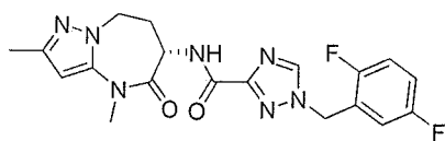
(S)-1-(2,5-difluorobenzyl)-N-(2,4-dimethyl-5-oxo-5,6,7,8-tetrahydro-4H-pyrazolo[1,5-a][1,3]diazepin-6-yl)-1H-1,2,4-triazole-3-carboxamide
