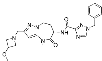
1-benzyl-N-[2-[(3-methoxyazetidin-1-yl)methyl]-4-methyl-5-oxo-7,8-dihydro-6H-pyrazolo[1,5-a][1,3]diazepin-6-yl]-1,2,4-triazole-3-carboxamide
