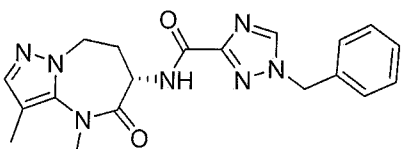
(S)-1-benzyl-N-(3,4-dimethyl-5-oxo-5,6,7,8-tetrahydro-4H-pyrazolo[1,5-a][1,3]diazepin-6-yl)-1H-1,2,4-triazole-3-carboxamide
