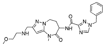
1-benzyl-N-[2-[(2-methoxyethylamino)methyl]-4-methyl-5-oxo-7,8-dihydro-6H-pyrazolo[1,5-a][1,3]diazepin-6-yl]-1,2,4-triazole-3-carboxamide
