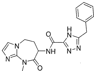
5-benzyl-N-(9-methyl-8-oxo-6,7,8,9-tetrahydro-5H-imidazo[1,2-a][1,3]diazepin-7-yl)-4H-1,2,4-triazole-3-carboxamide
