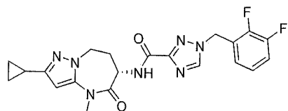
(S)-N-(2-cyclopropyl-4-methyl-5-oxo-5,6,7,8-tetrahydro-4H-pyrazolo[1,5-a][1,3]diazepin-6-yl)-1-(2,3-difluorobenzyl)-1H-1,2,4-triazole-3-carboxamide
