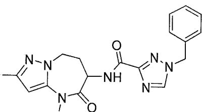
1-benzyl-N-(2,4-dimethyl-5-oxo-5,6,7,8-tetrahydro-4H-pyrazolo[1,5-a][1,3]diazepin-6-yl)-1H-1,2,4-triazole-3-carboxamide
