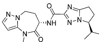
(5S)-5-isopropyl-N-[(6S)-4-methyl-5-oxo-7,8-dihydro-6H-pyrazolo[1,5-a][1,3]diazepin-6-yl]-6,7-dihydro-5H-pyrrolo[1,2-b][1,2,4]triazole-2-carboxamide
