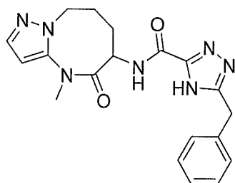
5-benzyl-N-(4-methyl-5-oxo-4,5,6,7,8,9-hexahydropyrazolo[1,5-a][1,3]diazocin-6-yl)-4H-1,2,4-triazole-3-carboxamide
