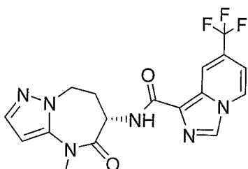
(S)-N-(4-methyl-5-oxo-5,6,7,8-tetrahydro-4H-pyrazolo[1,5-a][1,3]diazepin-6-yl)-7-(trifluoromethyl)imidazo[1,5-a]pyridine-1-carboxamide
