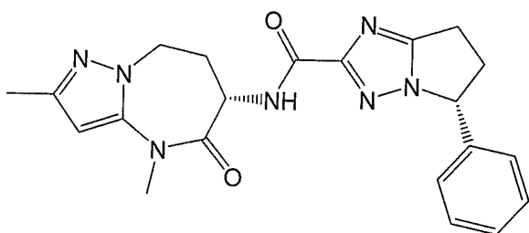
(5R)-5-phenyl-N-[(6S)-2,4-dimethyl-5-oxo-7,8-dihydro-6H-pyrazolo[1,5-a][1,3]diazepin-6-yl]-6,7-dihydro-5H-pyrrolo[1,2-b][1,2,4]triazole-2-carboxamide, and
