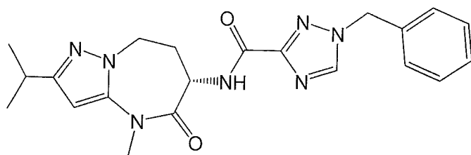
(S)-1-benzyl-N-(2-isopropyl-4-methyl-5-oxo-5,6,7,8-tetrahydro-4H-pyrazolo[1,5-a][1,3]diazepin-6-yl)-1H-1,2,4-triazole-3-carboxamide,
