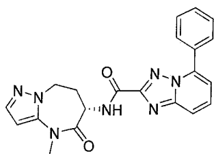
N-[(6S)-4-methyl-5-oxo-7,8-dihydro-6H-pyrazolo[1,5-a][1,3]diazepin-6-yl]-5-phenyl-[1,2,4]triazolo[1,5-a]pyridine-2-carboxamide
