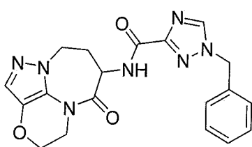
1-benzyl-N-(6-oxo-4,5,6,7,8,9-hexahydro-3-oxa-1,5a,9a-triazabenzocd]azulen-7-yl)-1H-1,2,4-triazole-3-carboxamide
