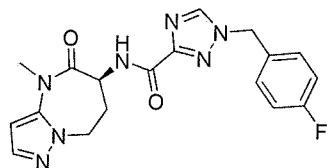
1-[(4-fluorophenyl)methyl]-N-[rac-(6S)-4-methyl-5-oxo-7,8-dihydro-6H-pyrazolo[1,5-a][1,3]diazepin-6-yl]-1,2,4-triazole-3-carboxamide
