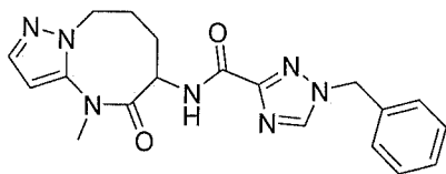
1-benzyl-N-(4-methyl-5-oxo-4,5,6,7,8,9-hexahydropyrazolo[1,5-a][1,3]diazocin-6-yl)-1H-1,2,4-triazole-3-carboxamide
