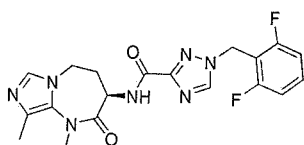
1-[(2,6-difluorophenyl)methyl]-N-(3R)-1,9-dimethyl-2-oxo-4,5-dihydro-3H-imidazo[1,5-a][1,3]diazepin-3-yl-1,2,4-triazole-3-carboxamide
