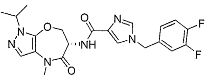
(S)-1-(3,4-difluorobenzyl)-N-(1-isopropyl-4-methyl-5-oxo-4,5,6,7-tetrahydro-1H-pyrazolo[3,4-b][1,4]oxazepin-6-yl)-1H-imidazole-4-carboxamide
