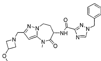
1-benzyl-N-[2-[(3-methoxyazetidin-1-yl)methyl]-4-methyl-5-oxo-7,8-dihydro-6H-pyrazolo[1,5-a][1,3]diazepin-6-yl]-1,2,4-triazole-3-carboxamide
