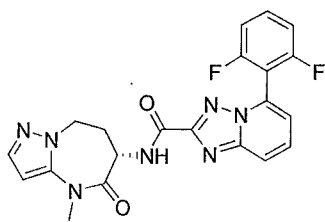
5-(2,6-difluorophenyl)-N-[(6S)-4-methyl-5-oxo-7,8-dihydro-6H-pyrazolo[1,5-a][1,3]diazepin-6-yl]-[1,2,4]triazolo[1,5-a]pyridine-2-carboxamide
