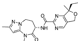
rac-(7R)-7-ethyl-7-methyl-N-[rac-(6S)-2,4-dimethyl-5-oxo-7,8-dihydro-6H-pyrazolo[1,5-a][1,3]diazepin-6-yl]-5H-furo[3,4-d]pyrimidine-2-carboxamide
