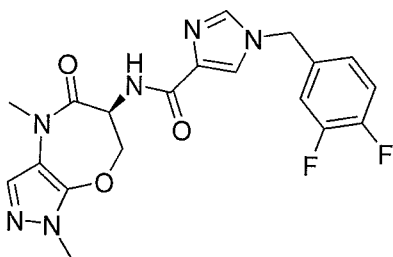
(S)-1-(3,4-difluorobenzyl)-N-(1,4-dimethyl-5-oxo-4,5,6,7-tetrahydro-1H-pyrazolo[3,4-b][1,4]oxazepin-6-yl)-1H-imidazole-4-carboxamide
