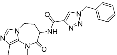
1-benzyl-N-(1,9-dimethyl-2-oxo-2,3,4,5-tetrahydro-1H-imidazo[1,5-a][1,3]diazepin-3-yl)-1H-1,2,3-triazole-4-carboxamide
