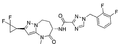
1-(2,3-difluorobenzyl)-N-((S)-2-((R)-2,2-difluorocyclopropyl)-4-methyl-5-oxo-5,6,7,8-tetrahydro-4H-pyrazolo[1,5-a][1,3]diazepin-6-yl)-1H-1,2,4-triazole-3-carboxamide
