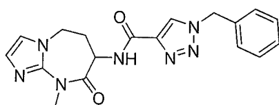
1-benzyl-N-(9-methyl-8-oxo-6,7,8,9-tetrahydro-5H-imidazo[1,2-a][1,3]diazepin-7-yl)-1H-1,2,3-triazole-4-carboxamide
