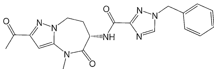
(S)-N-(2-acetyl-4-methyl-5-oxo-5,6,7,8-tetrahydro-4H-pyrazolo[1,5-a][1,3]diazepin-6-yl)-1-benzyl-1H-1,2,4-triazole-3-carboxamide,
