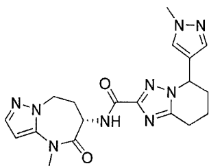
5-(1-methylpyrazol-4-yl)-N-[rac-(6S)-4-methyl-5-oxo-7,8-dihydro-6H-pyrazolo[1,5-a][1,3]diazepin-6-yl]-5,6,7,8-tetrahydro-[1,2,4]triazolo[1,5-a]pyridine-2-
