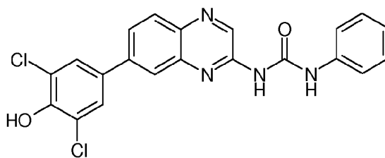
1-[7-(3,5-Dichloro-4-hydroxy-phenyl)-quinoxalin-2-yl]-3-phenyl-urea (Compound 86)
