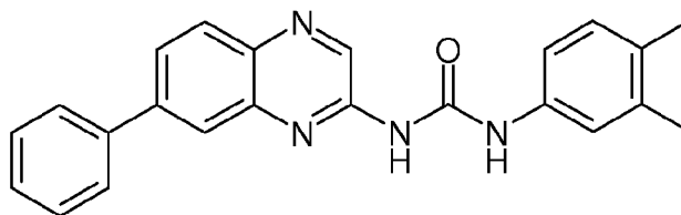
1-(3,4-dimethylphenyl)-3-(7-phenylquinoxalin-2-yl)urea ( Compound 28 )
