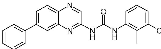
1-(3-chloro-2-methylphenyl)-3-(7-phenylquinoxalin-2-yl)urea ( Compound 27 )
