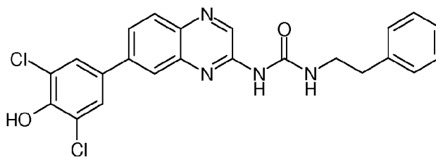
1-[7-(3,5-Dichloro-4-hydroxy-phenyl)-quinoxalin-2-yl]-3-phenethyl-urea (Compound 85)
