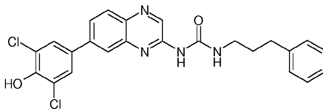
1-[7-(3,5-Dichloro-4-hydroxy-phenyl)-quinoxalin-2-yl]-3-(3-phenyl-propyl)-urea (Compound 84)
