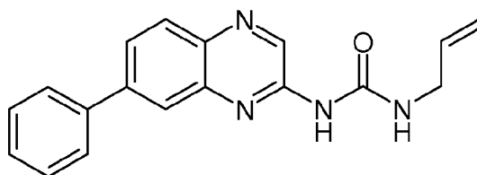
1-allyl-3-(7-phenylquinoxalin-2-yl)urea ( Compound 29 )
