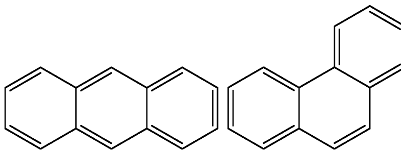
anthracene
