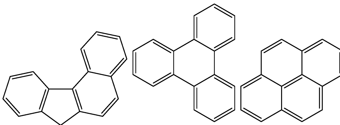
benzo(c)fluorene
