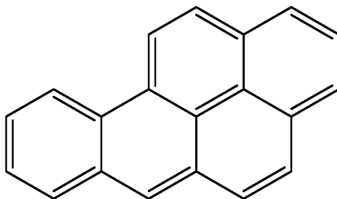
benzo(a)pyrene
