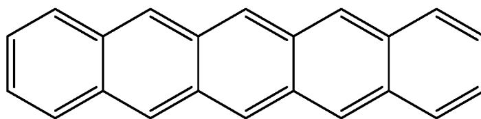
pentacene
