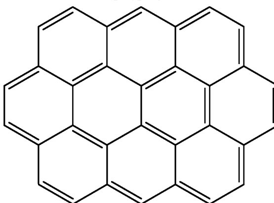
ovalene
