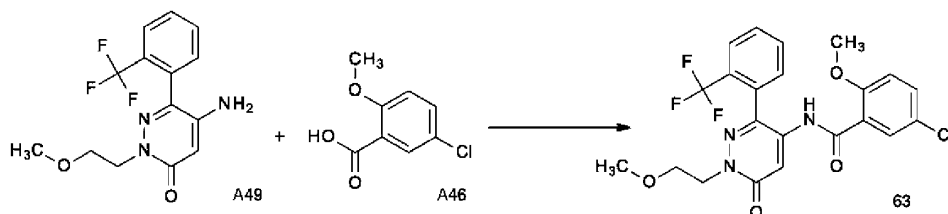
Scheme 29
