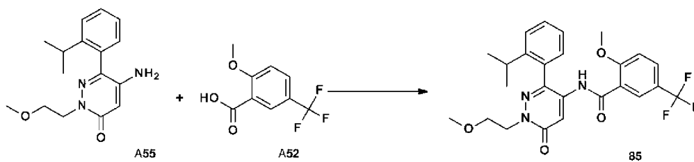
Scheme 39
