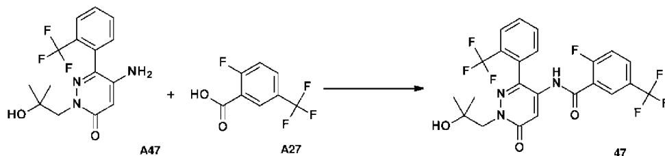
Scheme 27
