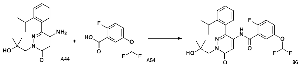
Scheme 40
