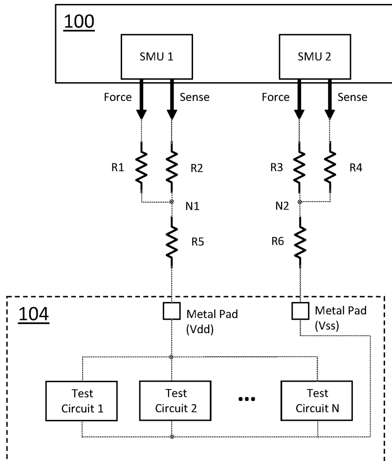
FIG. 5 (Prior Art)
