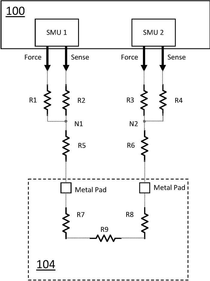
FIG. 4 (Prior Art)
