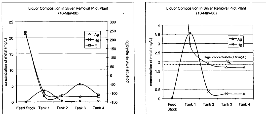
Figure 3: Profile of Silver Removal v Tanks
