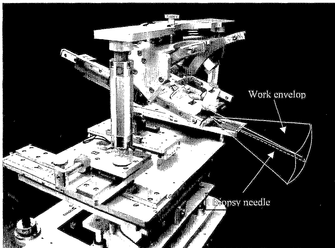
FIG. 8 Inventors' previous biopsy robot system design
