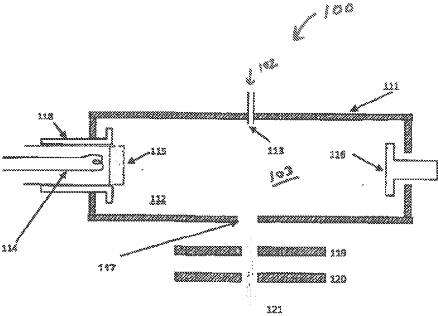
Schematic of an ion source apparatus
