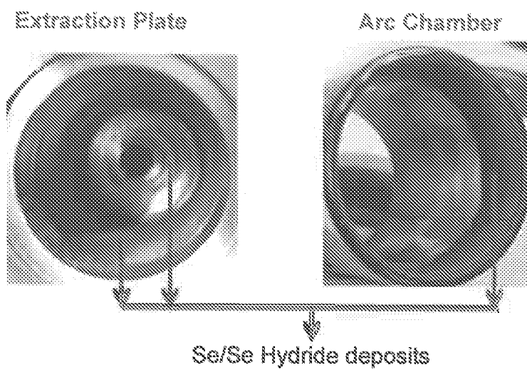
Figure 3a and 3b: Deposits during H_2Se Implant
