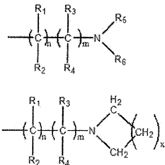
aminoalkyls
