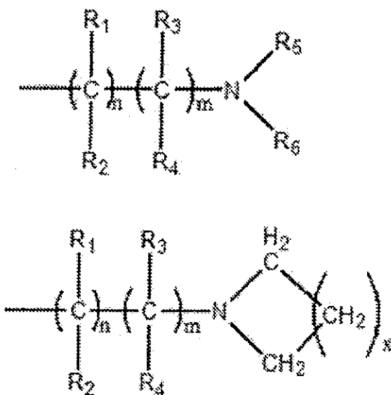
aminoalkyls
