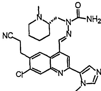
(S)-(-)-6
