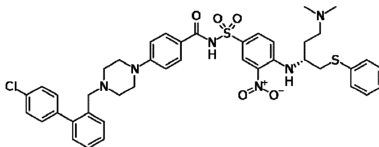
Formula III: ABT-737
