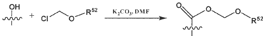
Scheme 7
