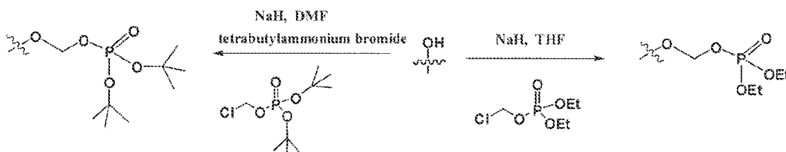
Scheme 6
