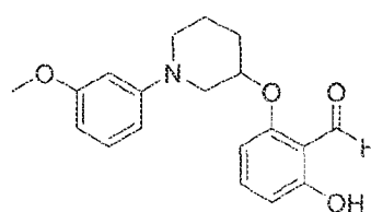
2-hydroxy-6-((1-(3-methoxyphenyl)piperidin-3-yl)oxy)benzaldehyde
