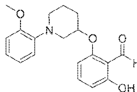
2-hydroxy-6-((1-(2-methoxyphenyl)piperidin-3-yl)oxy)benzaldehyde
