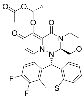
(I-1-1-2)
