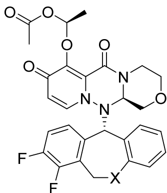
(I-1-1)
