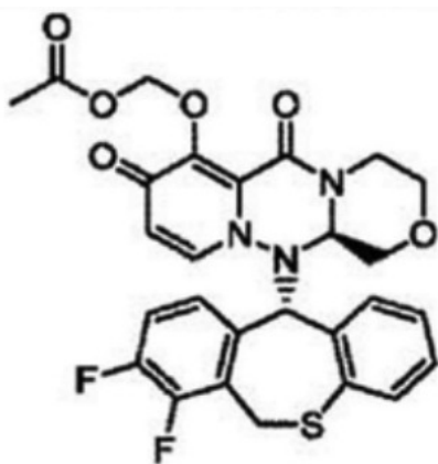
(II-5)
