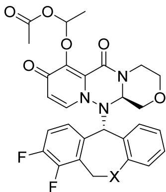
(I-1)
