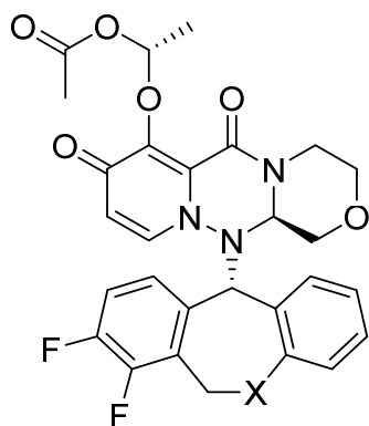
(I-1-2) ;
