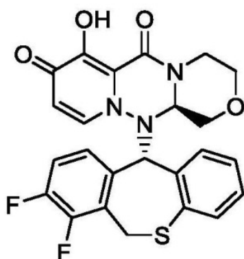
(Baloxavir)
