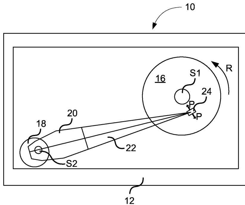
Figure 1B (Conventional)
