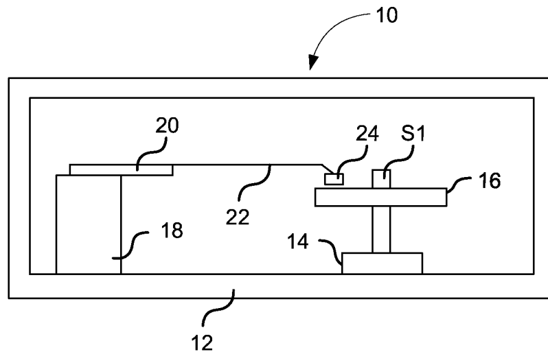
Figure 1A (Conventional)
