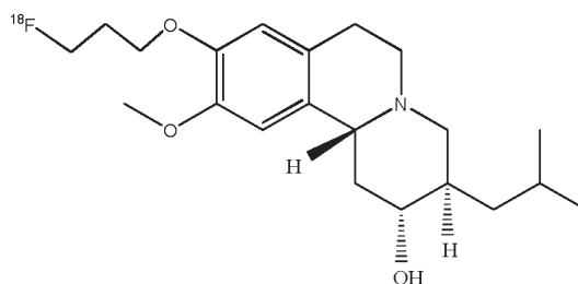
[ ^{18}\text{F} ]AV-133
