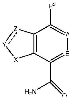
Formula (I)
