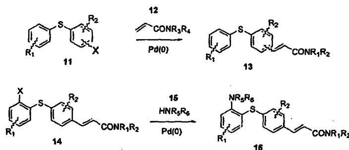
Scheme 4
