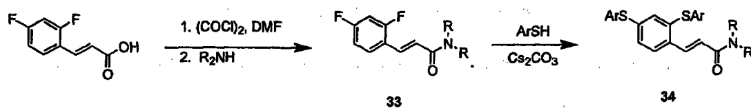
Scheme 8
