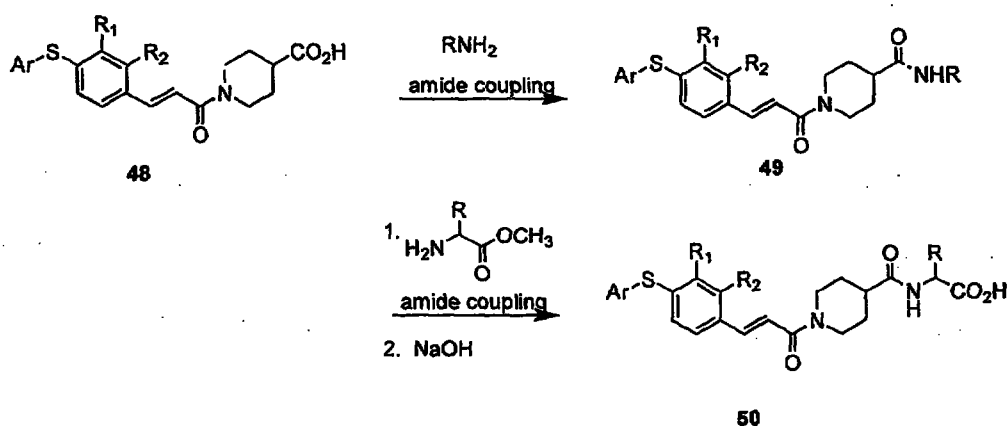
Scheme 12
