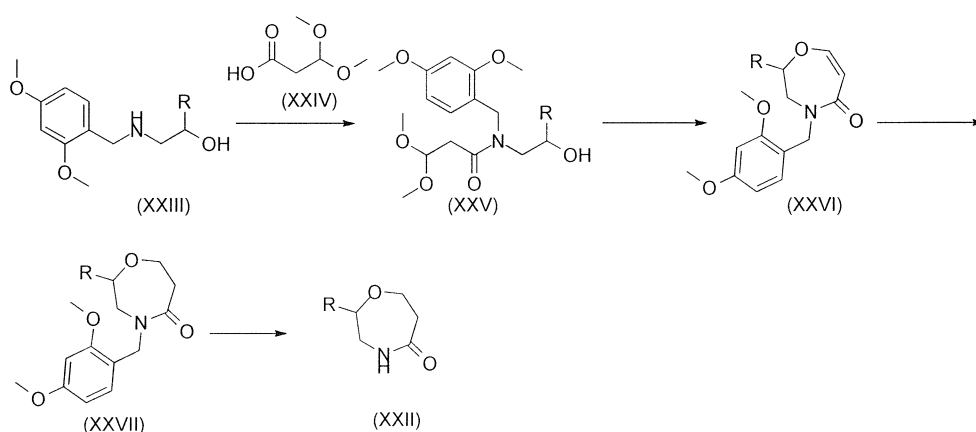
[0035] Scheme 8
