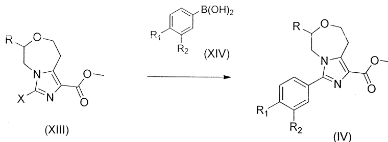
[0032] Scheme 5
