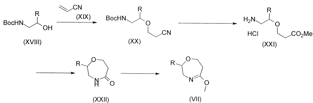
[0034] Scheme 7
