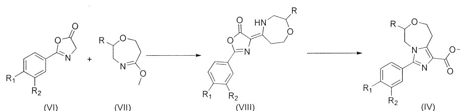
[0030] Scheme 3
