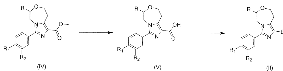
[0029] Scheme 2
