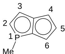
1-methylcyclopenta[b] phospholyl
