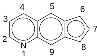
cyclopenta[g]quinolyl
