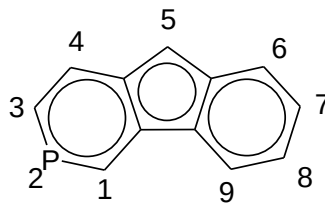
indeno[1,2-c]phosphinyl
