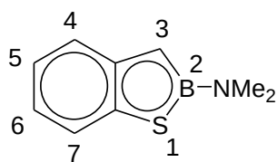
2-dimethylamino- 1,2-benzothiaborollide
