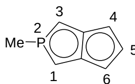
2-methylcyclopenta[c] phospholyl
