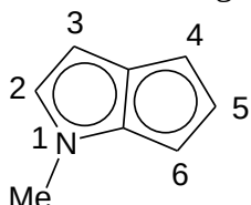
1-methylcyclopenta[b]pyrrolyl
