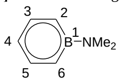
1-dimethylamino-boratabenzene
