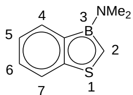
3-dimethylamino- 1,3-benzothiaborollide
