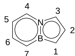
3a,7a-azaborindenyl
