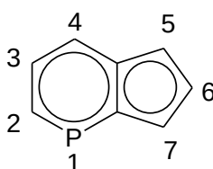
cyclopenta[b]phosphinyl
