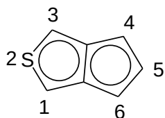
cyclopenta[c]thienyl
