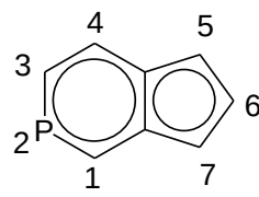
cyclopenta[c]phosphinyl
