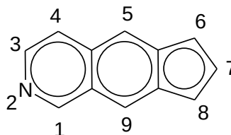
cyclopenta[g]isoquinolyl
