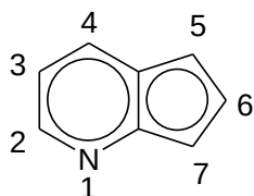
cyclopenta[b]pyridyl
