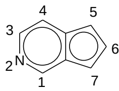
cyclopenta[c]pyridyl
