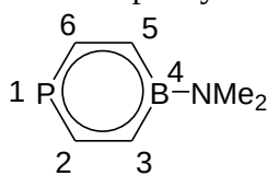
4-dimethylamino-1,4-phosphaboratabenzene
