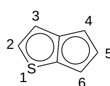
cyclopenta[b]thienyl
