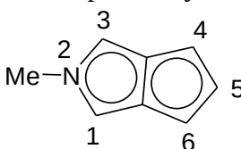
2-methylcyclopenta[c]pyrrolyl
