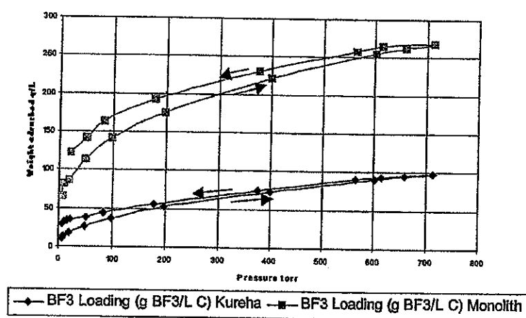
BF 3 Adsorption on Kureha BAC & PVDC char Monolith
