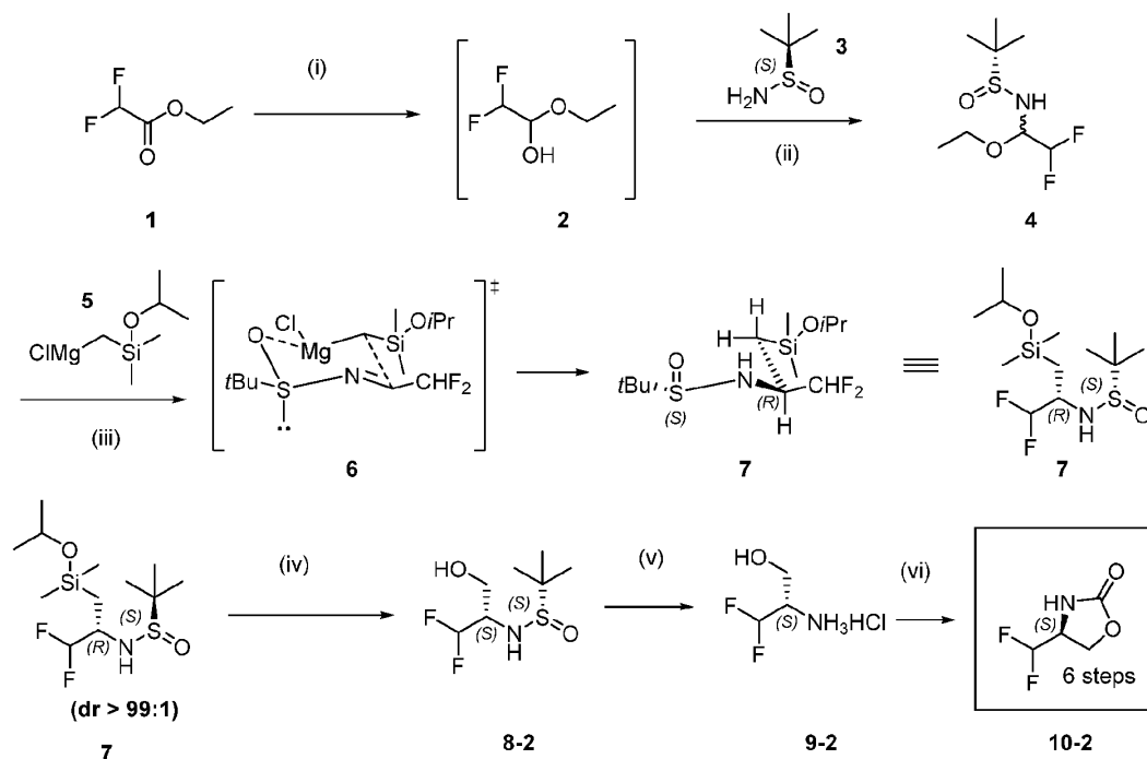
Scheme 1: Synthesis of Compound (10-2) by a Grignard-Tamoa Route
