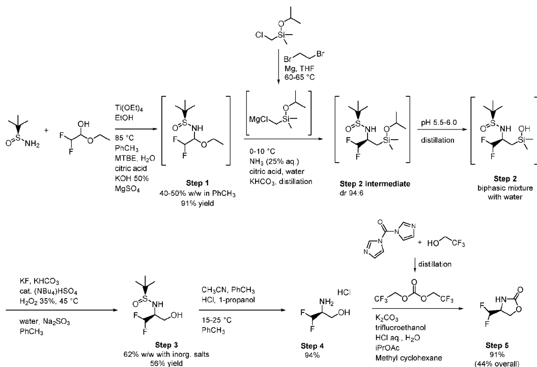
Scheme 1A: Alternative synthesis of Compound (10-2) by a Grignard-Tamoa Route
