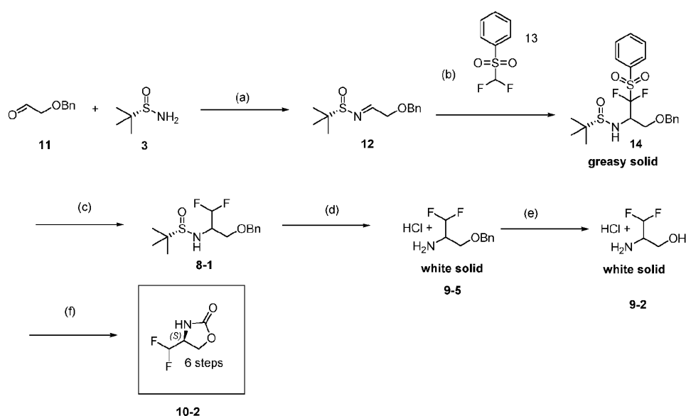
Scheme 4: Synthesis of Compound ( 10-2 ) by a Sulfone Route
