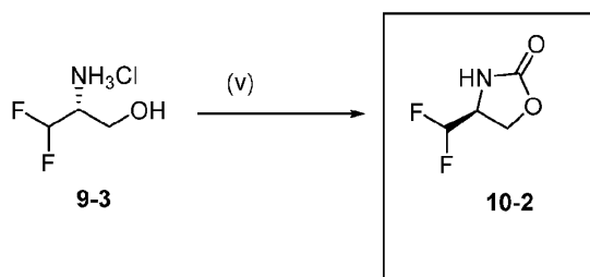
Scheme 3 Step (v):
