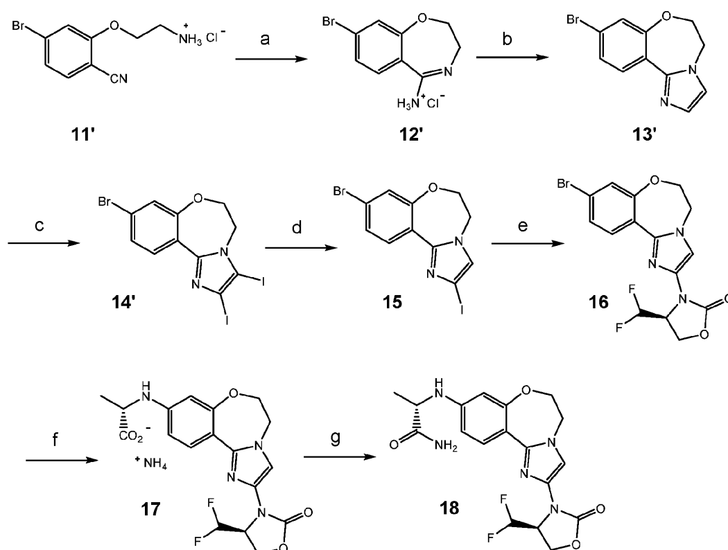
15 Scheme 5: Synthesis of Compound 18
