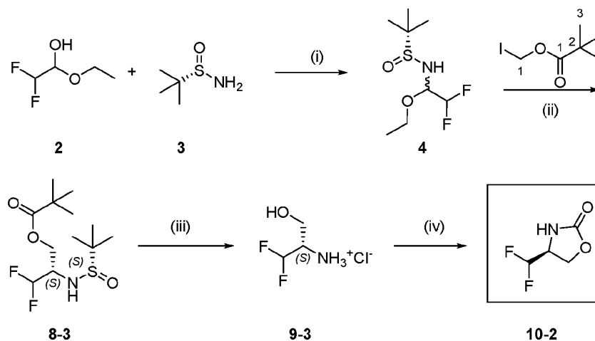
5 Scheme 2: Synthesis of Compound 10-2 by a Grignard-Knochel Route
