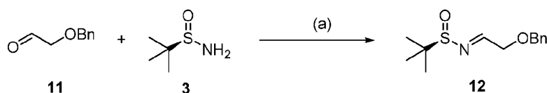
Scheme 4 Step (a):
