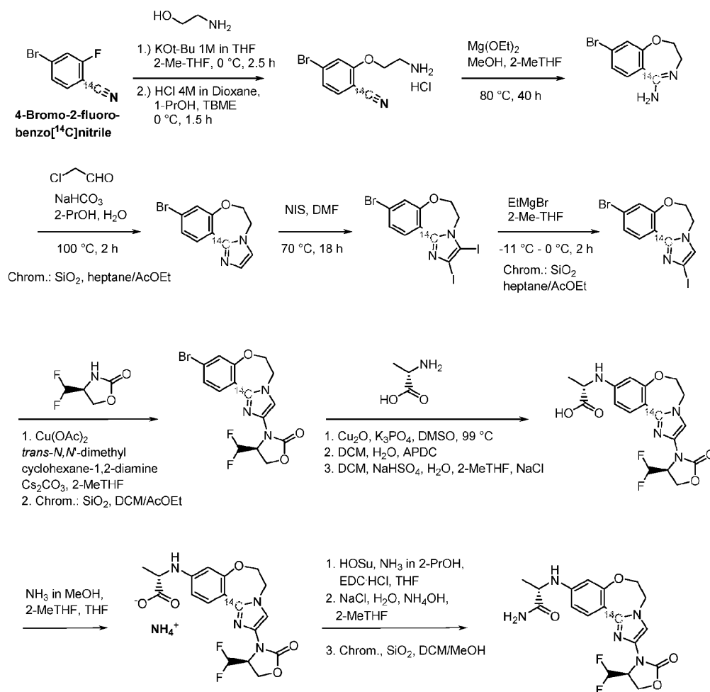
Scheme 6: Synthesis of ^{14}\text{C} labeled inavolisib
