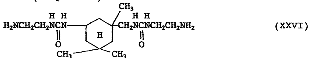
(Compound 10)
