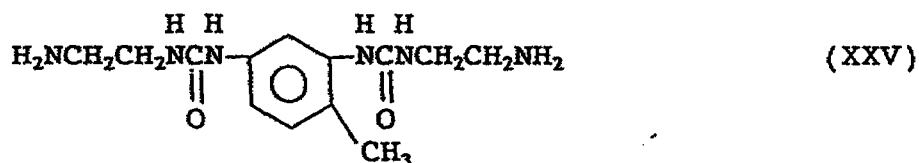
(Compound 9)
