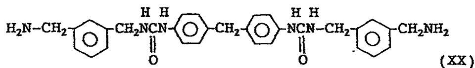
(Compound 4)
