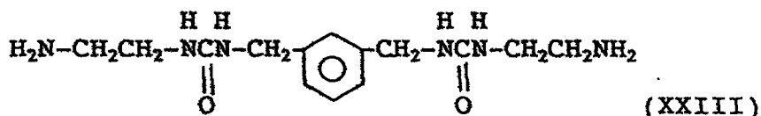
(Compound 7)
