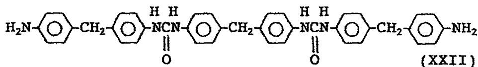
(Compound 6)
