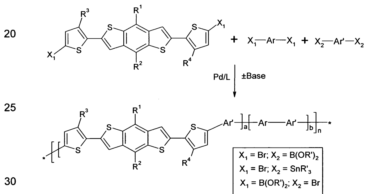
Scheme 6 - Synthesis of random co-polymers:
