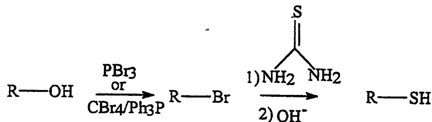
SCHEME B
