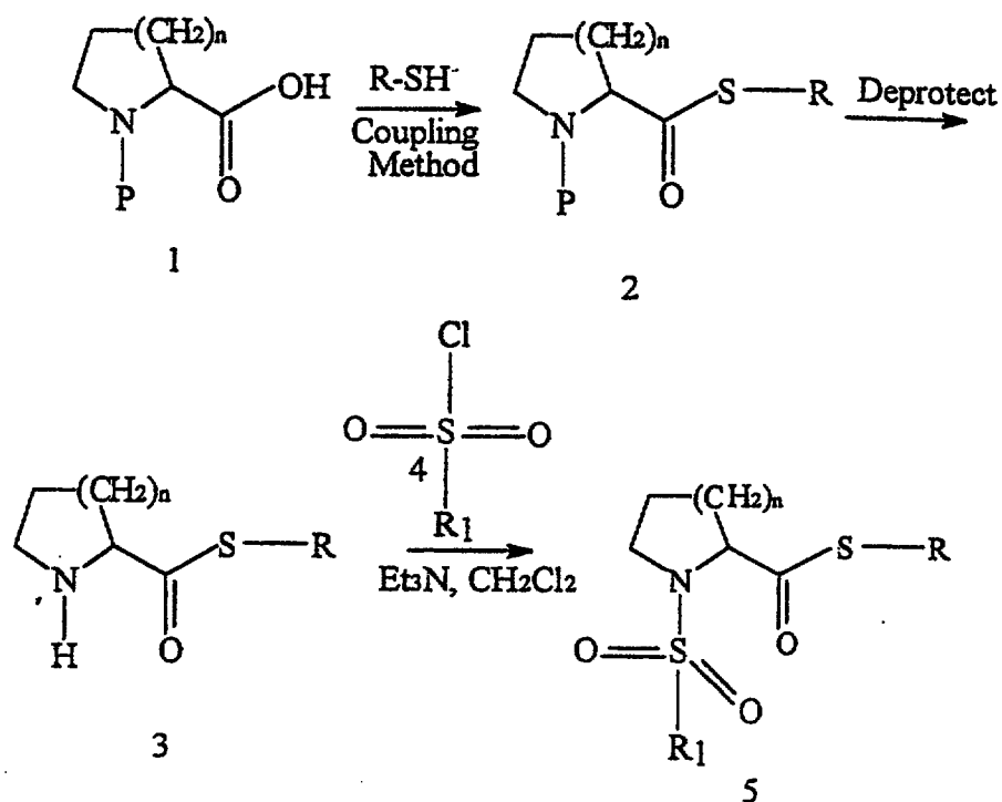
SCHEME A
