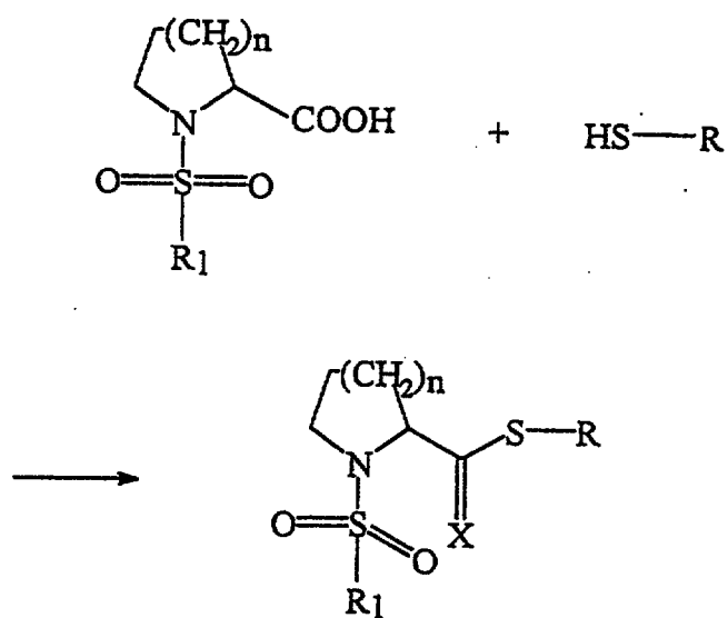
SCHEME C
