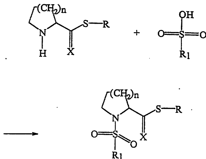
SCHEME D
