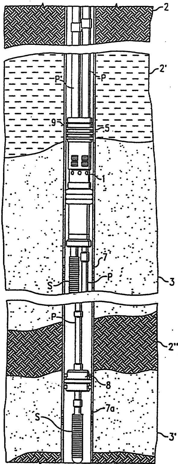
FIG. 1 (PRIOR ART)
