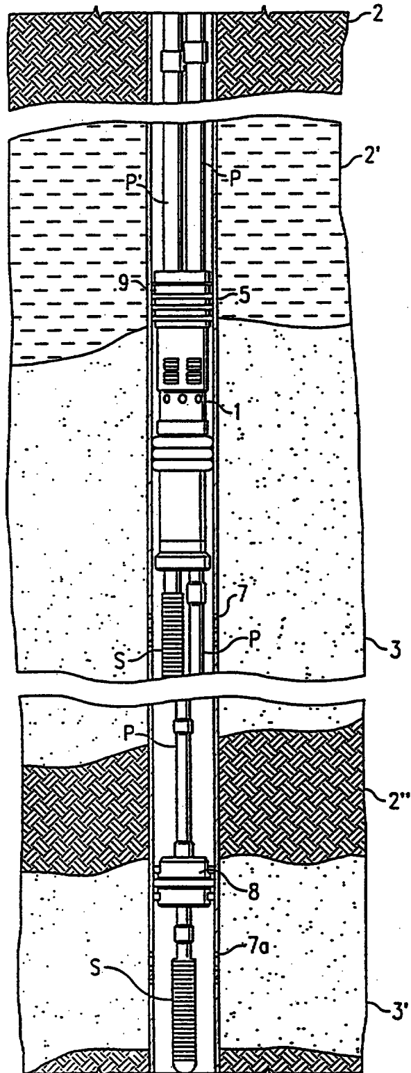
FIG. 1 (PRIOR ART)
