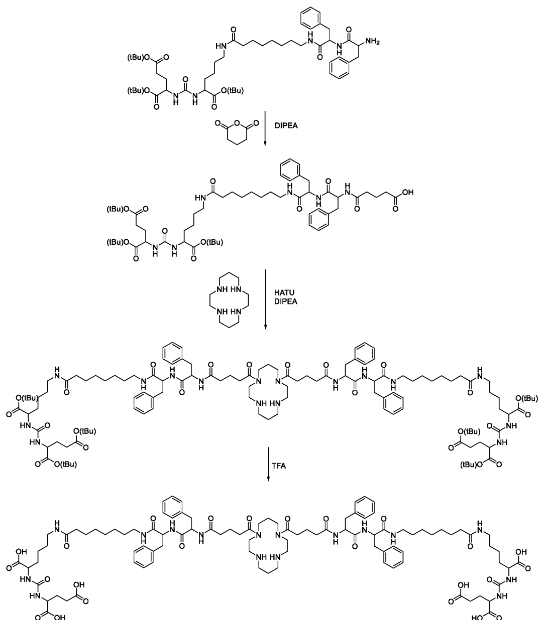
Scheme 2: Synthesis of compounds of Formula (I).
