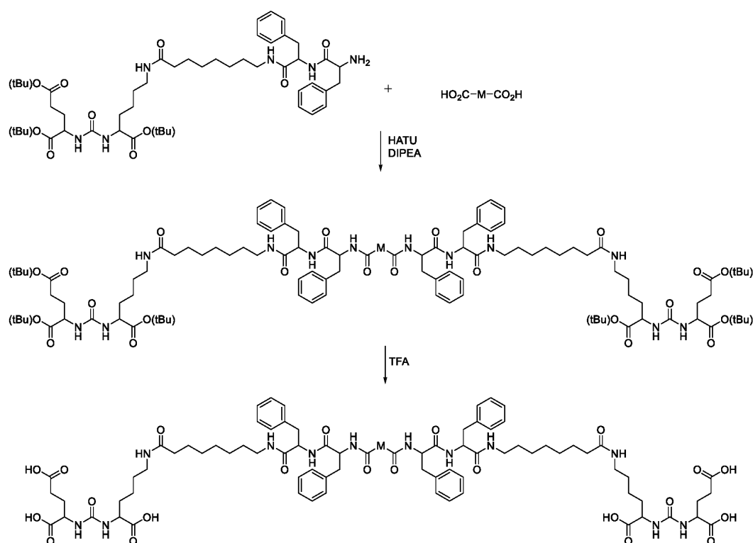
Scheme 1. Synthesis of compounds of Formula (I).
