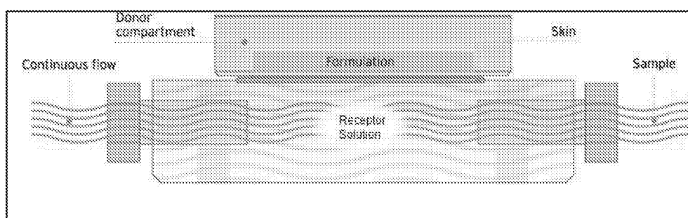
Schematic representation of MedFlux-HT™ cell Figure 3
