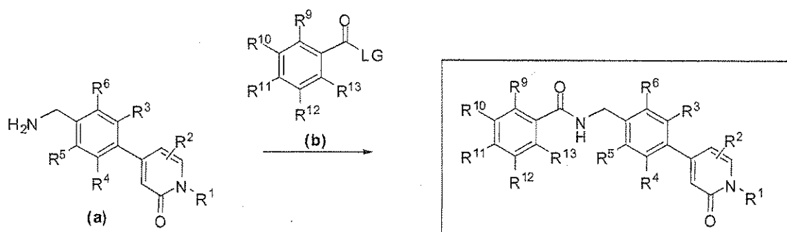
Scheme I
