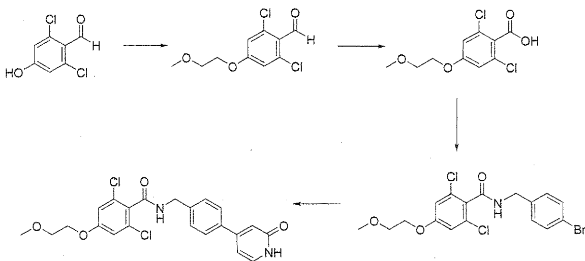
Scheme VII
