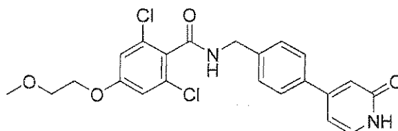
Scheme VII
