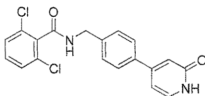
Scheme VIII
