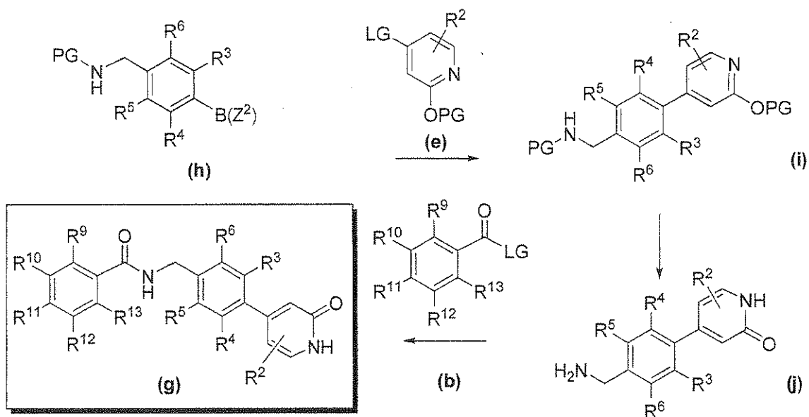
Scheme III
