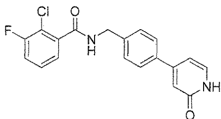
Scheme IX
