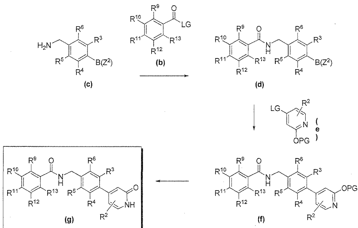
Scheme II
