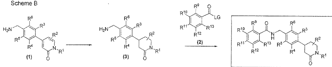
Scheme B
