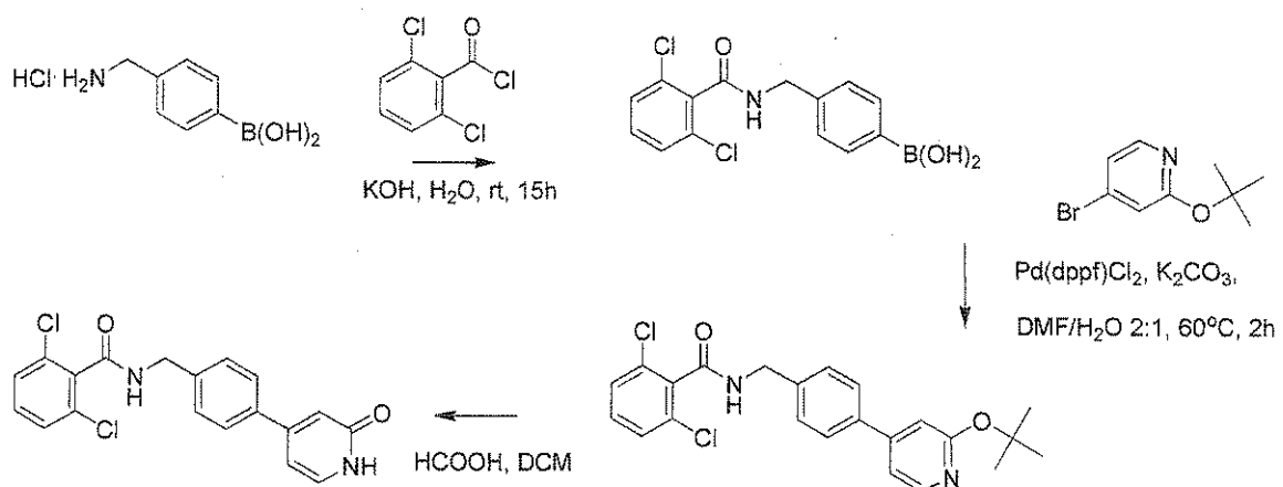
Scheme VIII
