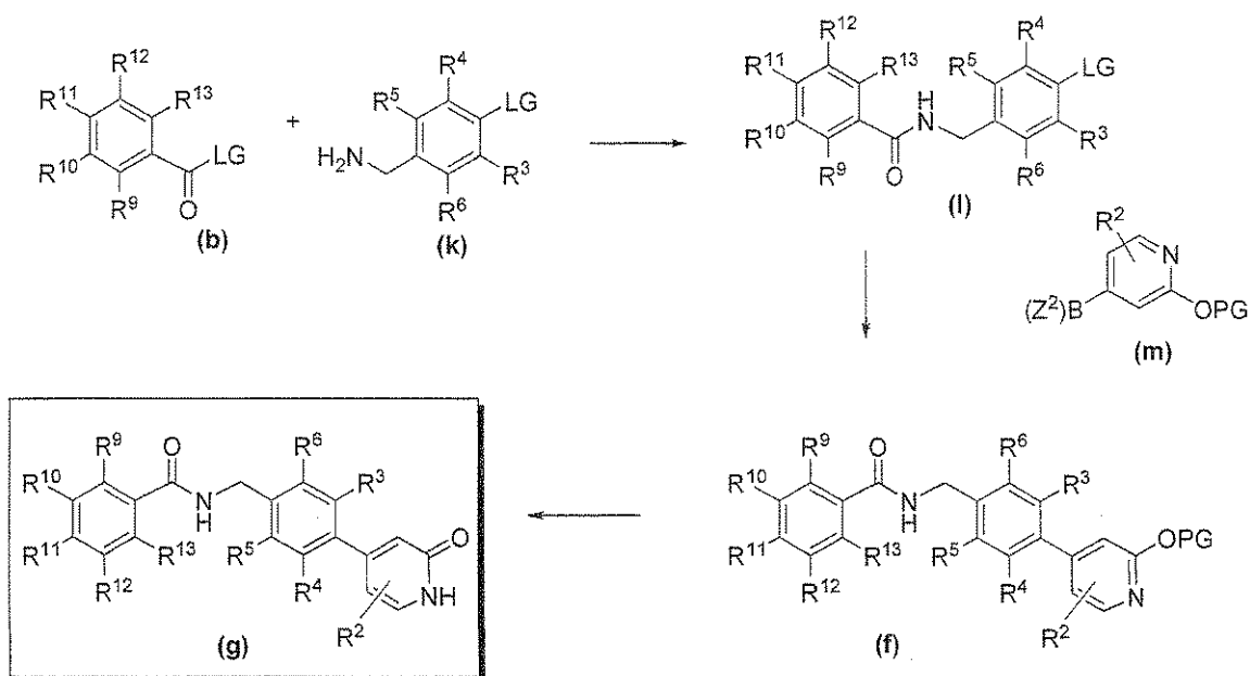
Scheme IV
