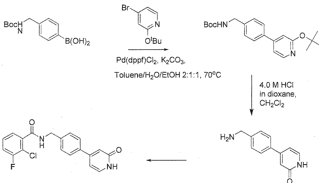
Scheme IX
