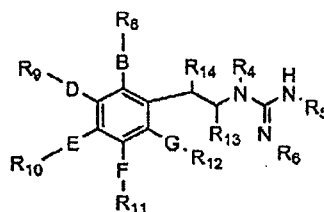
Structure Delta
