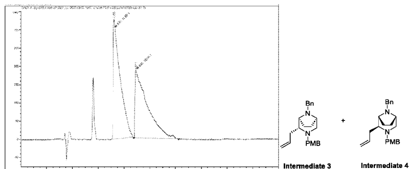
FIG. 1: Racemic mixture of Intermediates 3 and 4
