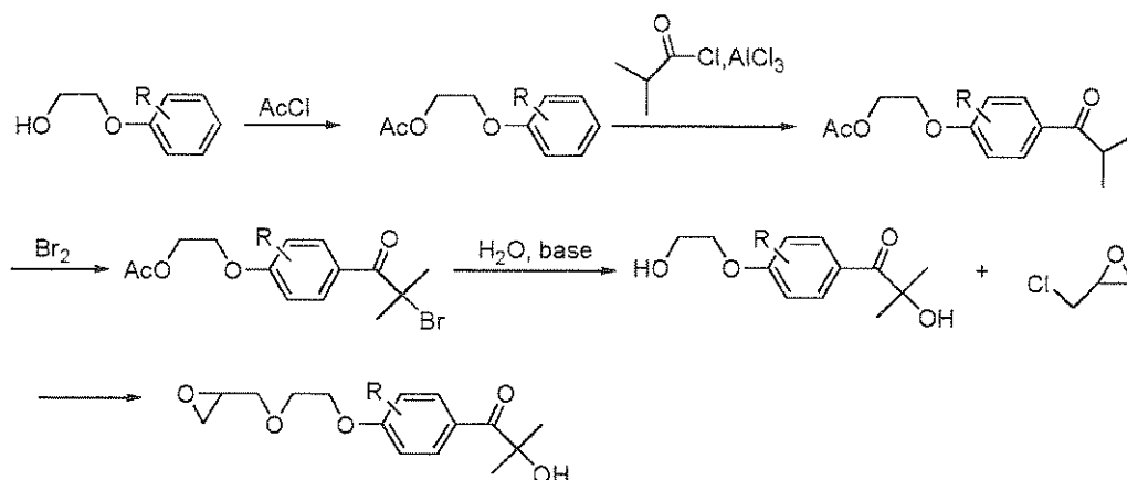
Scheme 4: Preparation of analogues of (3).
