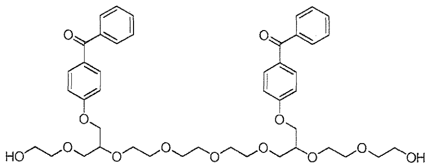
Scheme 1: Example of applying formula I to a photoinitiator. Formula I then reads
