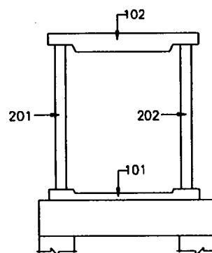
SECTION 1-1
