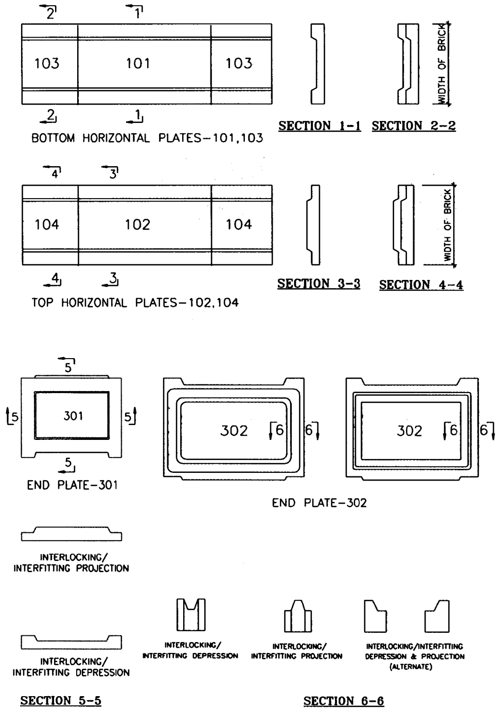
MOULD-6
