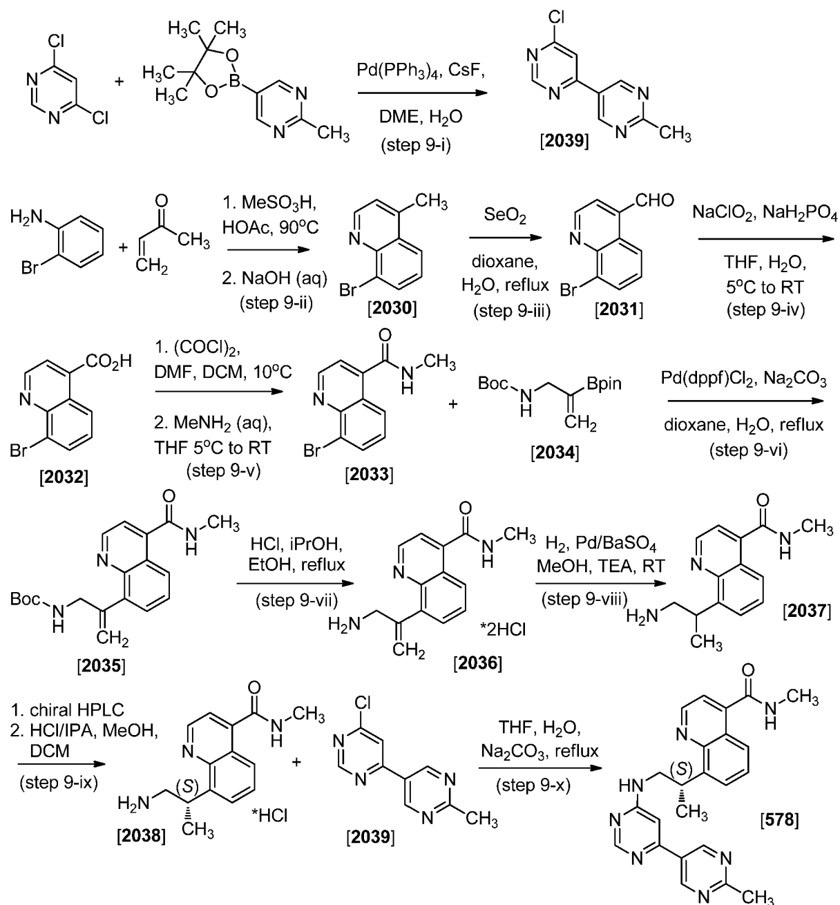
Scheme 9
