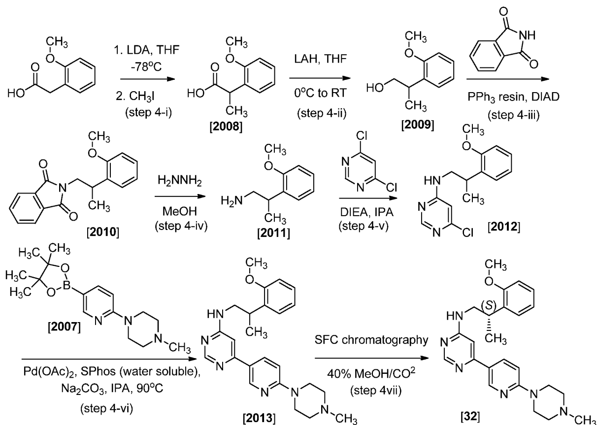
Scheme 4
