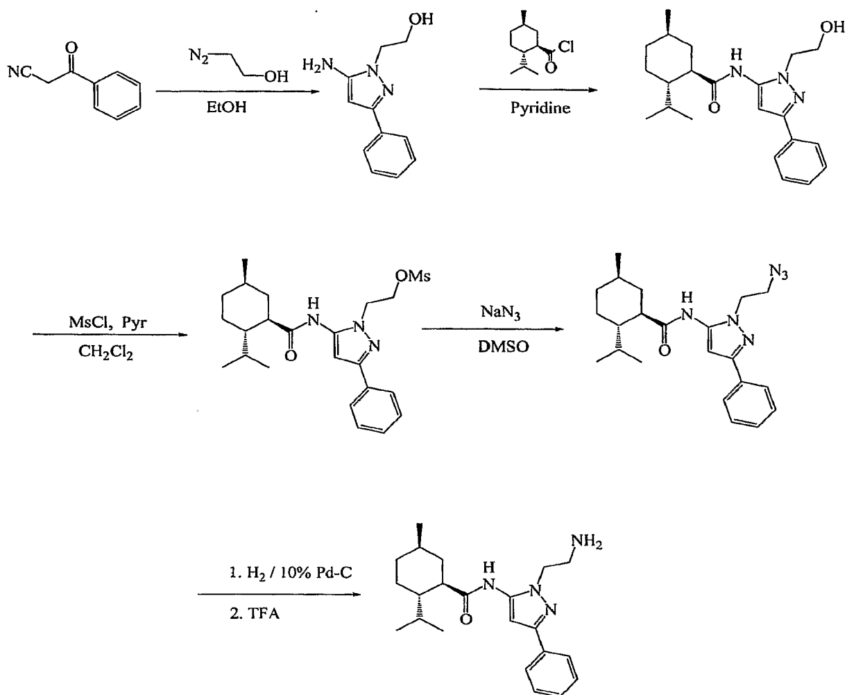
Scheme 5.
