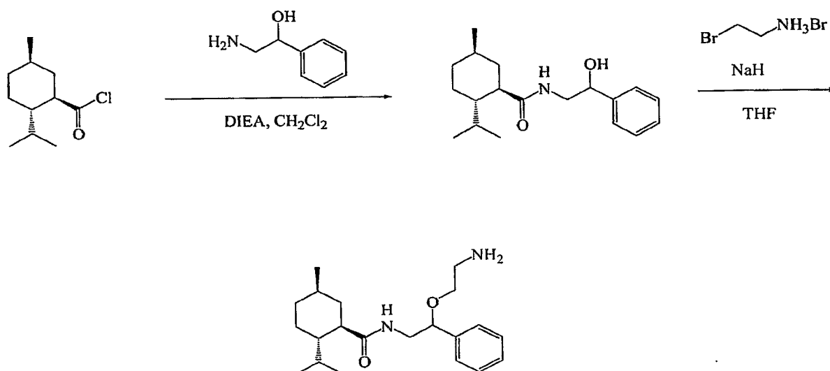
Scheme 6.
