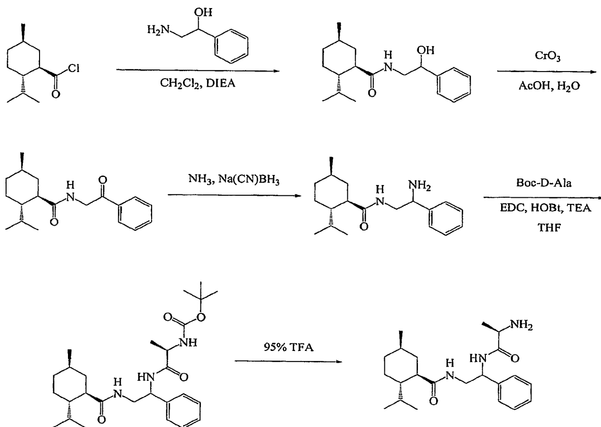
Scheme 7.
