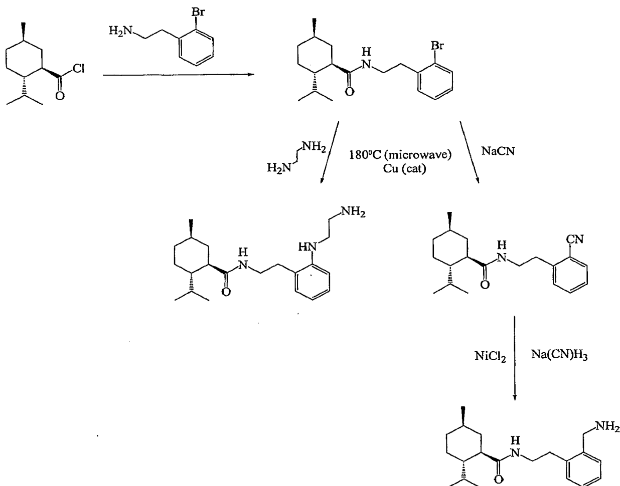
Scheme 7.
