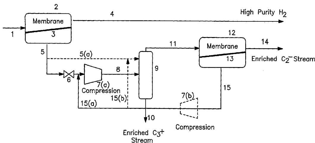
New Membrane Process for LPG Recovery
