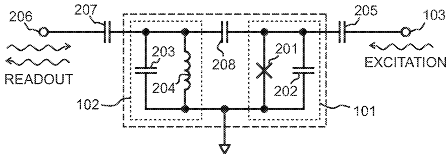
Fig. 2 PRIOR ART
