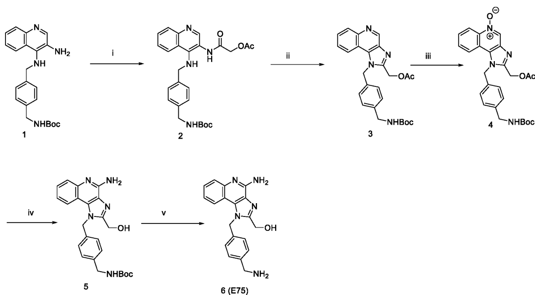
Scheme 4. Reagents: (i) AcOCH 2 COCl, NEt 3 , THF; (ii) Et 3 N, EtOH; (v) mCPBA, CHCl 3 ; (vi) Benzoyl isocyanate, CH 2 Cl 2 ; NaOH, MeOH (vii) 20% TFA, DCM, rt, 2h.
