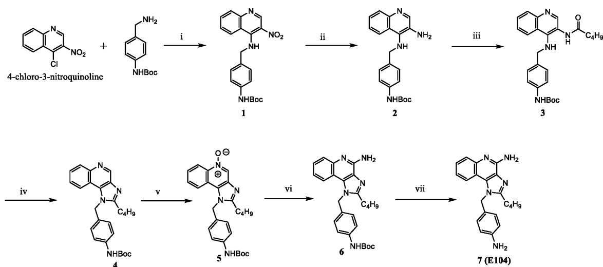
Scheme 2. Reagents: (i) \text{NEt}_3 , \text{CH}_2\text{Cl}_2 ; (ii) \text{Zn} , \text{HCOONH}_4 , \text{MeOH} ; (iii) \text{C}_4\text{H}_9\text{COCl} , \text{NEt}_3 , \text{THF} ; (iv) \text{NaOH} , \text{EtOH} ; (v) \text{mCPBA} , \text{CHCl}_3 ; (vi) Tosyl chloride, \text{CH}_2\text{Cl}_2 ; \text{NH}_4\text{OH} (vii) 20% \text{TFA} , \text{DCM} , rt, 2h.
