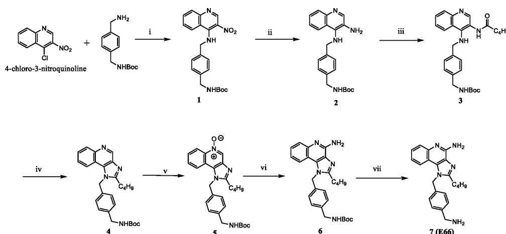
Scheme 1. Reagents: (i) NEt 3 , CH 2 Cl 2 ; (ii) Zn, HCOONH 4 , MeOH; (iii) C 4 H 9 COCl, NEt 3 , THF; (iv) NaOH, EtOH; (v) mCPBA, CHCl 3 ; (vi) Benzoyl isocyanate, CH 2 Cl 2 ; NaOH, MeOH (vii) 20% TFA, DCM, rt, 2h.
