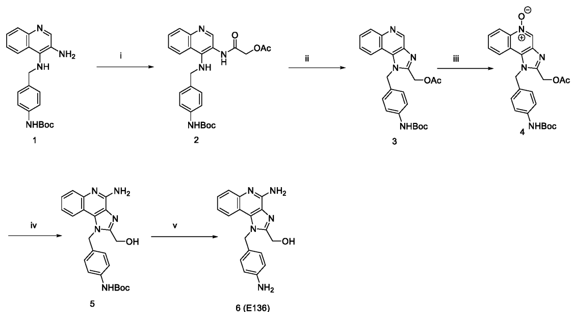
Scheme 3. Reagents: (i) \text{AcOCH}_2\text{COCl} , \text{NEt}_3 , THF; (ii) \text{Et}_3\text{N} , EtOH; (iv) mCPBA, \text{CHCl}_3 ; (v) Benzoyl isocyanate, \text{CH}_2\text{Cl}_2 ; NaOH, MeOH (vii) 20% TFA, DCM, rt, 2h.
