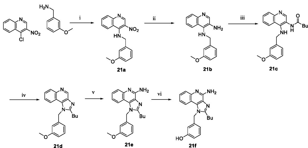
Scheme 1: Reagents (i) \text{RNH}_2 , \text{NEt}_3 , \text{CH}_2\text{Cl}_2 ; (ii) \text{Zn} , \text{HCOONH}_4 , \text{MeOH} ; (iii) \text{C}_6\text{H}_4\text{COCl} , \text{NEt}_3 , \text{EtOAc} ; (iv). \text{NaOH} , \text{EtOH}:\text{Water} (13:2); (v) a. \text{mCPBA} , \text{CHCl}_3 ; b. \text{NH}_4\text{OH}/\text{NH}_3 , \text{CHCl}_3 ; (vi). \text{BBr}_3 , \text{CH}_2\text{Cl}_2
