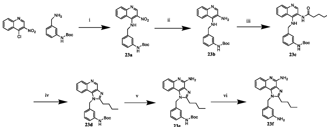
Scheme 1: Reagents (i) RNH 2 , NEt 3 , CH 2 Cl 2 ; (ii) Zn, HCOONH 4 , MeOH; (iii) C 4 H 9 COCl, NEt 3 , EtOAc; (iv) NaOH, EtOH:water (13:2); (v) a. mCPBA, CHCl 3 ; b. NH 4 OH/NH 3 , CHCl 3 ; (vi) 20% TFA, CH 2 Cl 2
