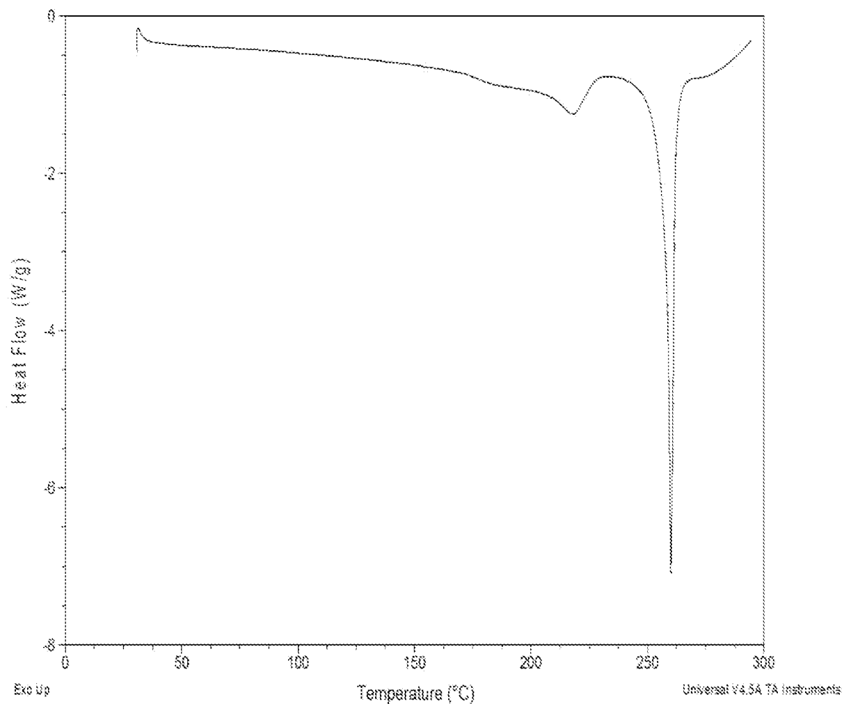
FIGURE 3a: DSC Compound I-1 (ethanol solvate)
