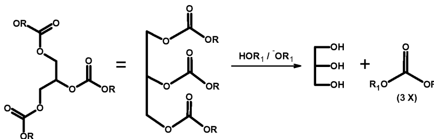
Scheme 1. Illustrative transesterification of triglycerides with methanol (HOR 1 ) with catalytic OH - to make biodiesel.
