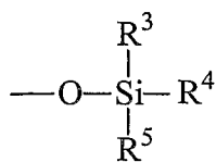
Formula IIIa
